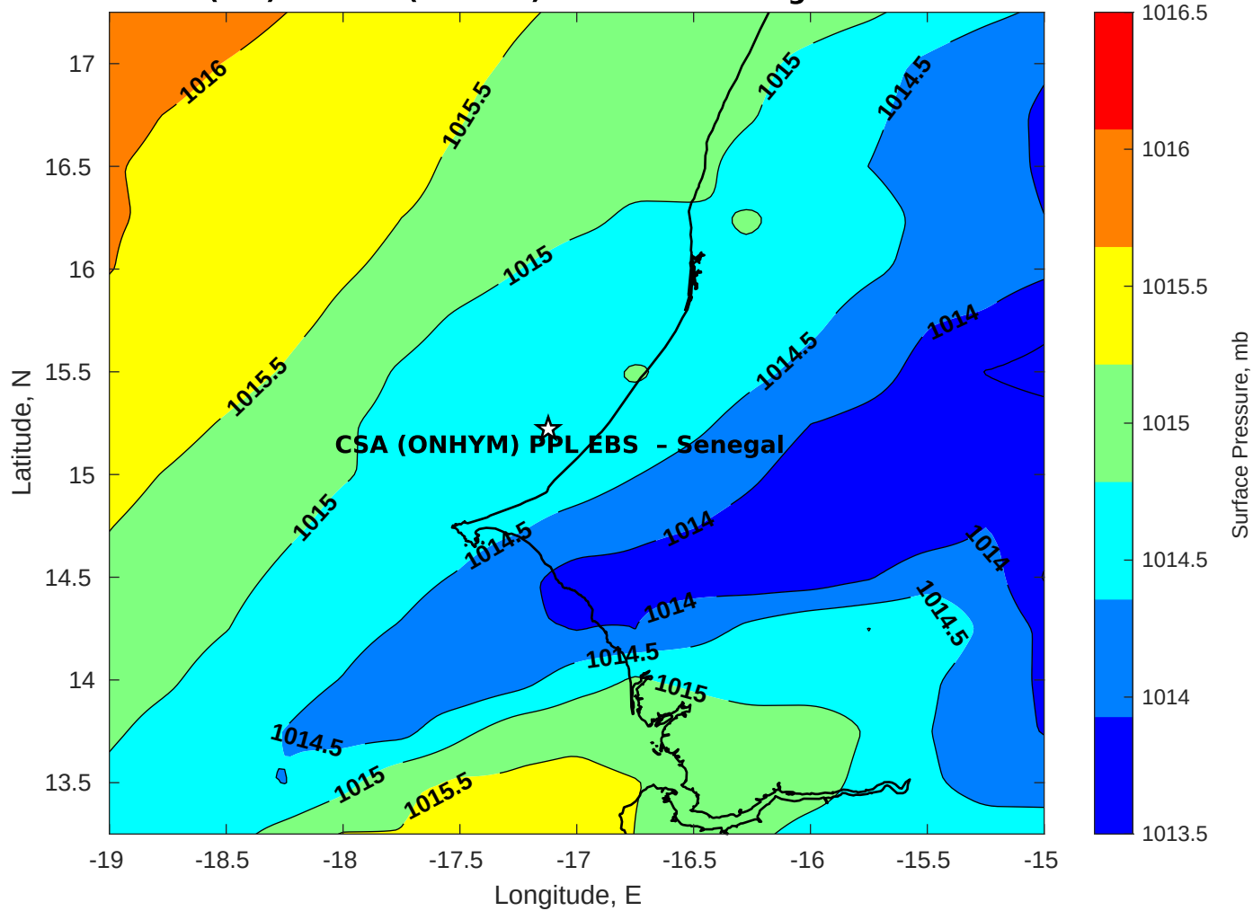
Surface Pressure (mb) for CSA (ONHYM) PPL EBS - Senegal at 05-Feb-2026 00:00:00
