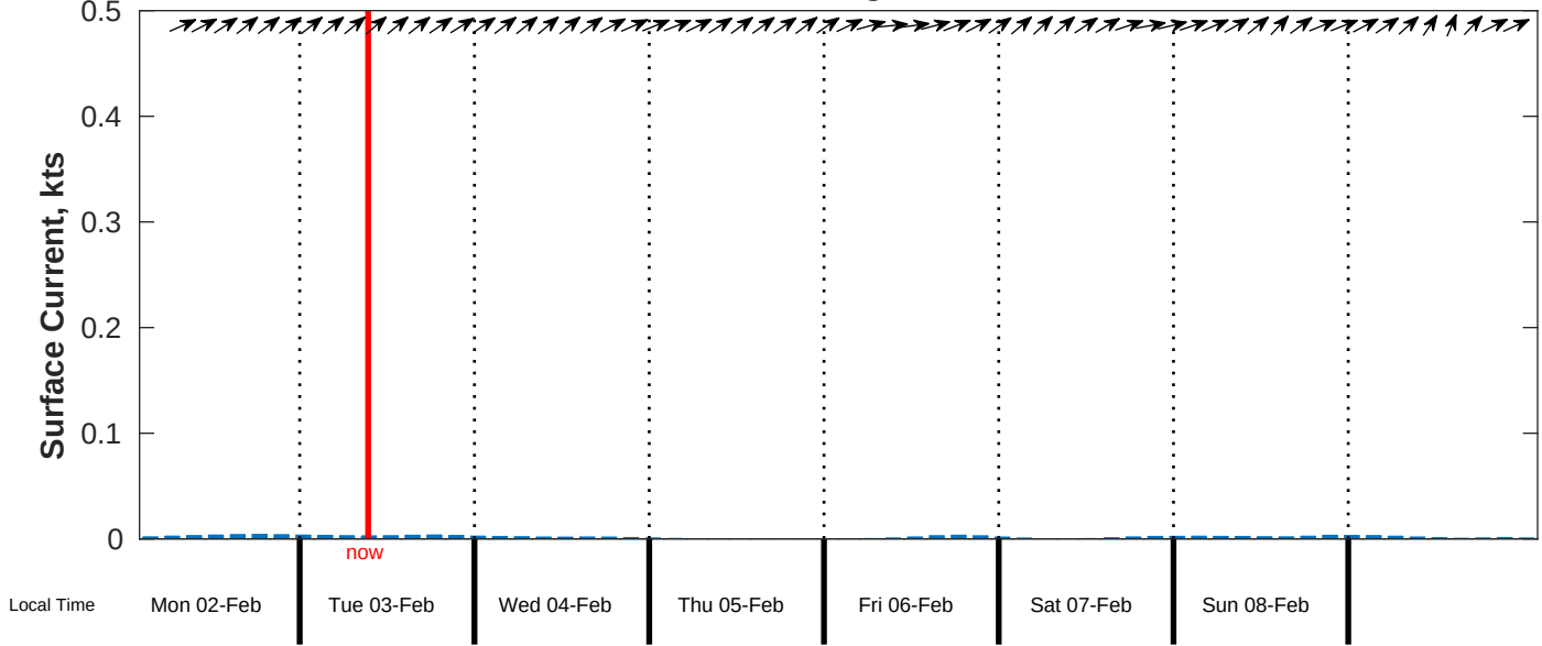
Surface Current Forecast for CSA (ONHYM) PPL EBS - Senegal from 02-Feb-2026 00:00:00 to 10-Feb-2026 00:00:00
