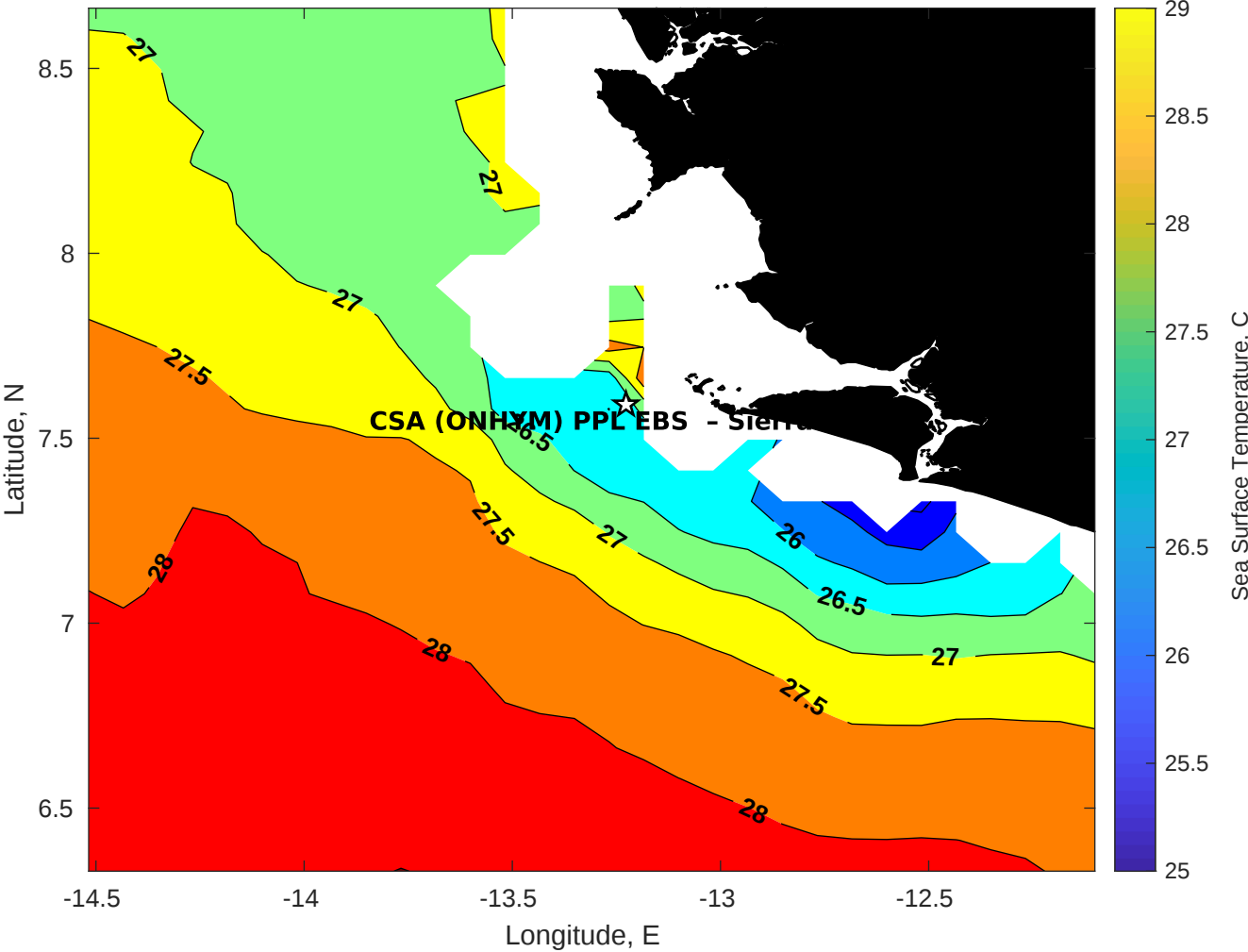
SST for CSA (ONHYM) PPL EBS - Sierra Leone at 02-Feb-2026 00:00:00
