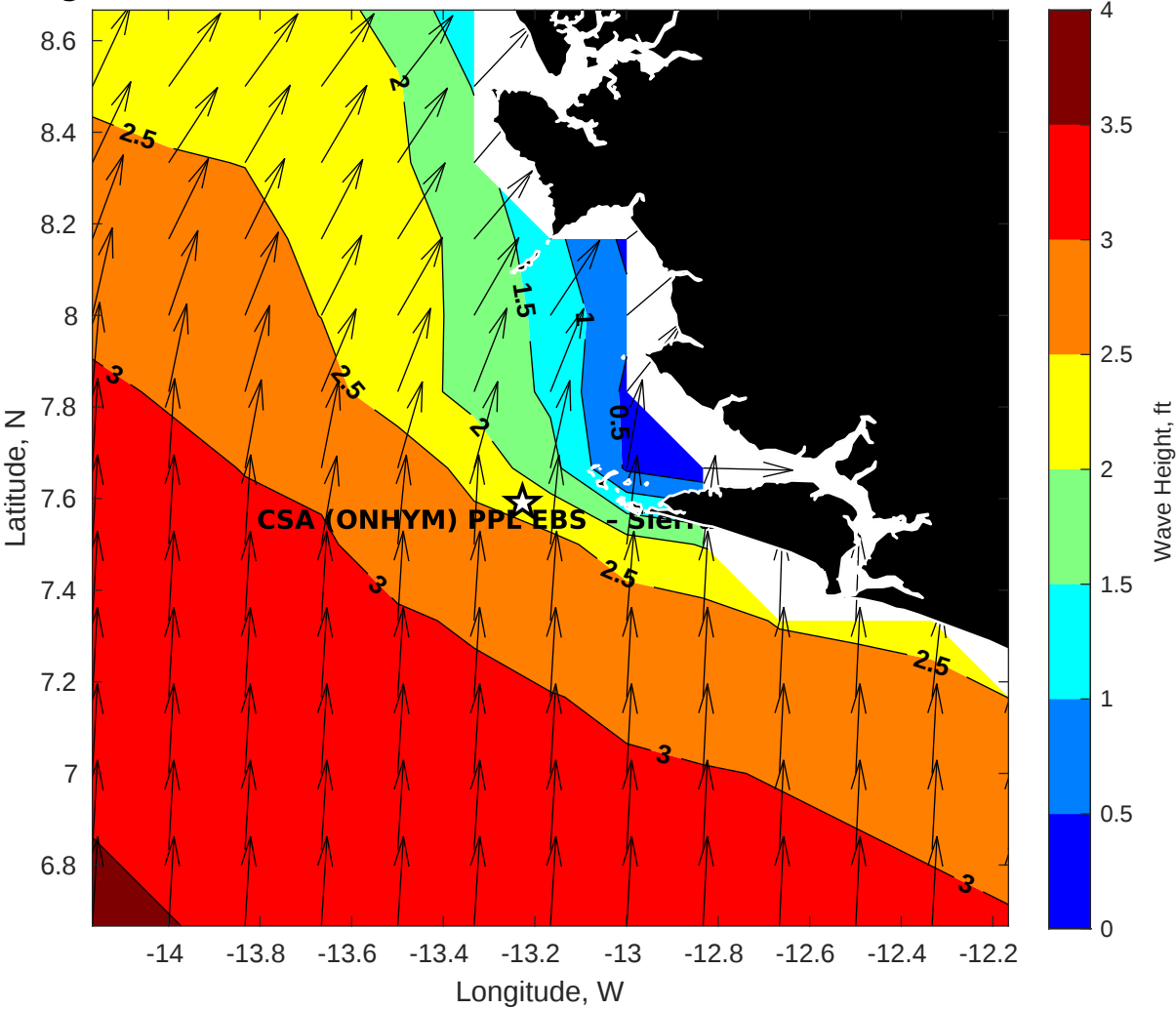
GFS Wave Height (ft) for CSA (ONHYM) PPL EBS - Sierra Leone at 03-Feb-2026 09:00:00
