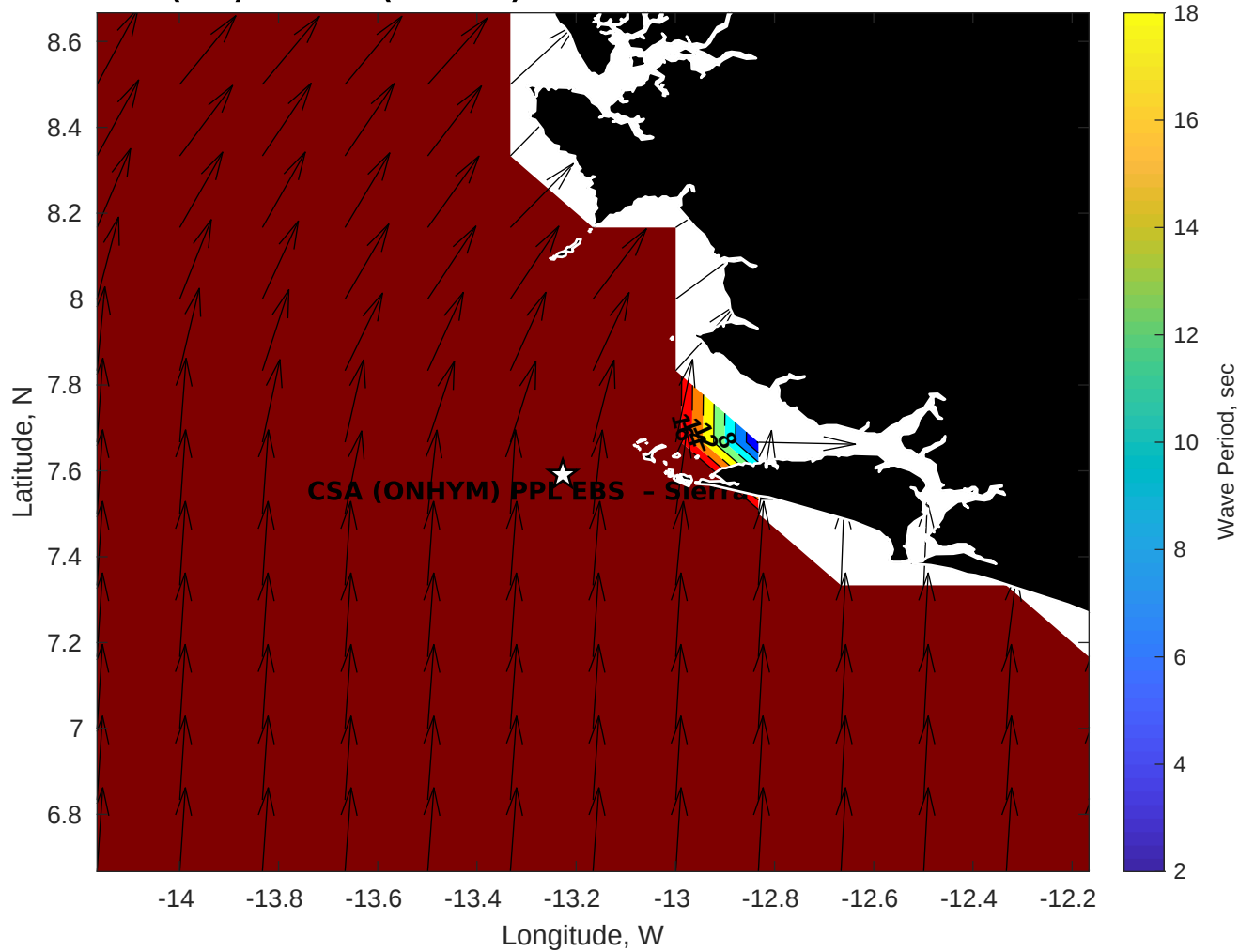
GFS Wave Period (sec) for CSA (ONHYM) PPL EBS - Sierra Leone at 03-Feb-2026 09:00:00
