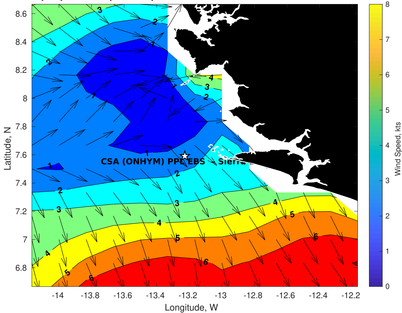
GFS Winds (kts) for CSA (ONHYM) PPL EBS - Sierra Leone at 03-Feb-2026 09:00:00
