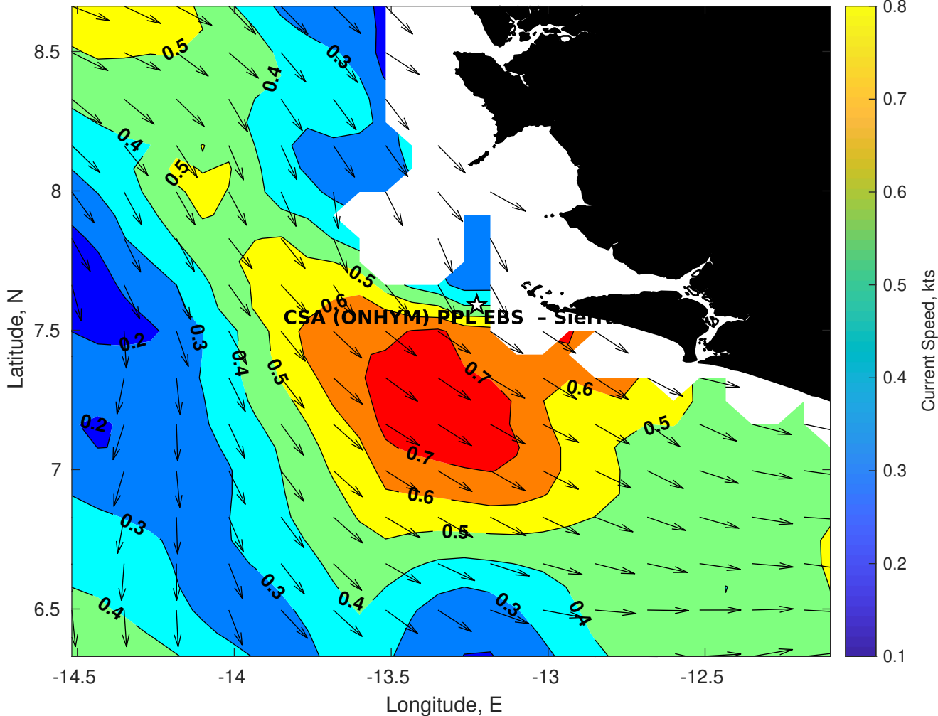
Surface Currents for CSA (ONHYM) PPL EBS - Sierra Leone at 02-Feb-2026 00:00:00
