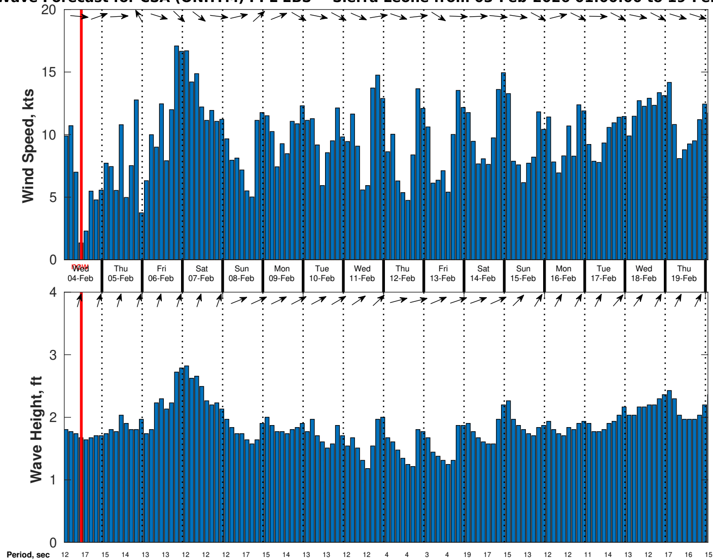
Wind & Wave Forecast for CSA (ONHYM) PPL EBS - Sierra Leone from 03-Feb-2026 01:00:00 to 19-Feb-2026 01:00:00
