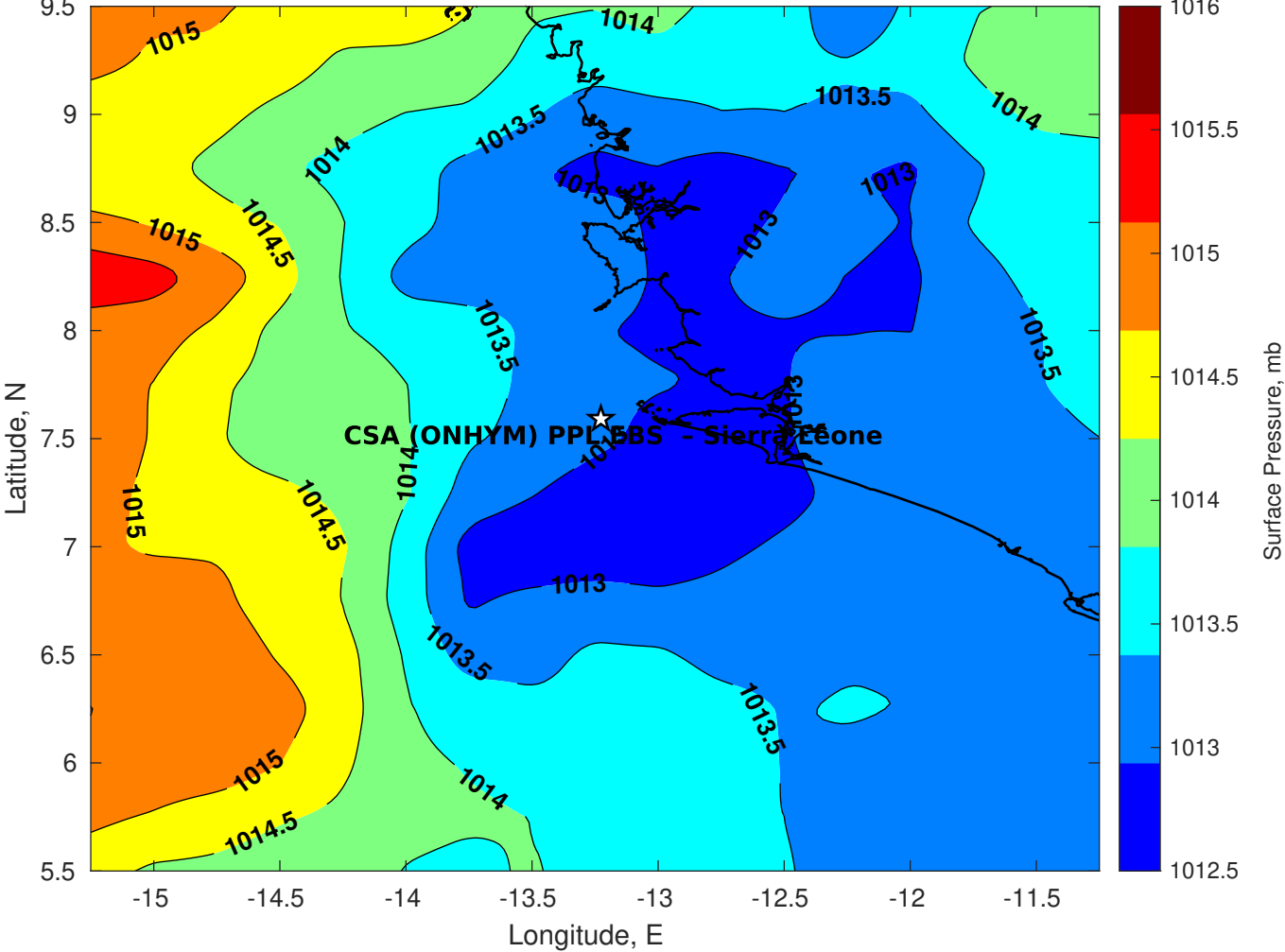
Surface Pressure (mb) for CSA (ONHYM) PPL EBS - Sierra Leone at 05-Feb-2026 00:00:00
