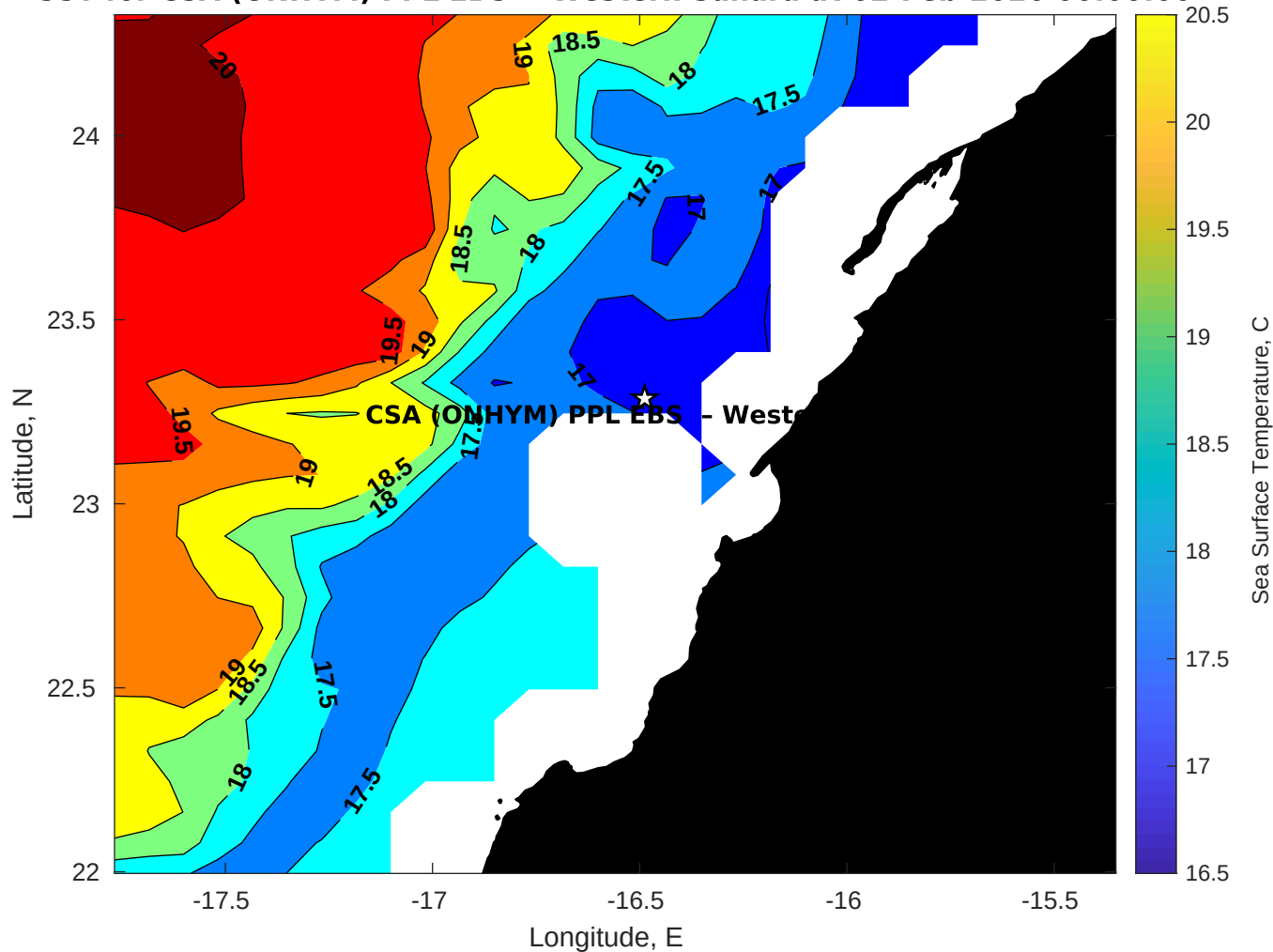
SST for CSA (ONHYM) PPL EBS - Western Sahara at 02-Feb-2026 00:00:00
