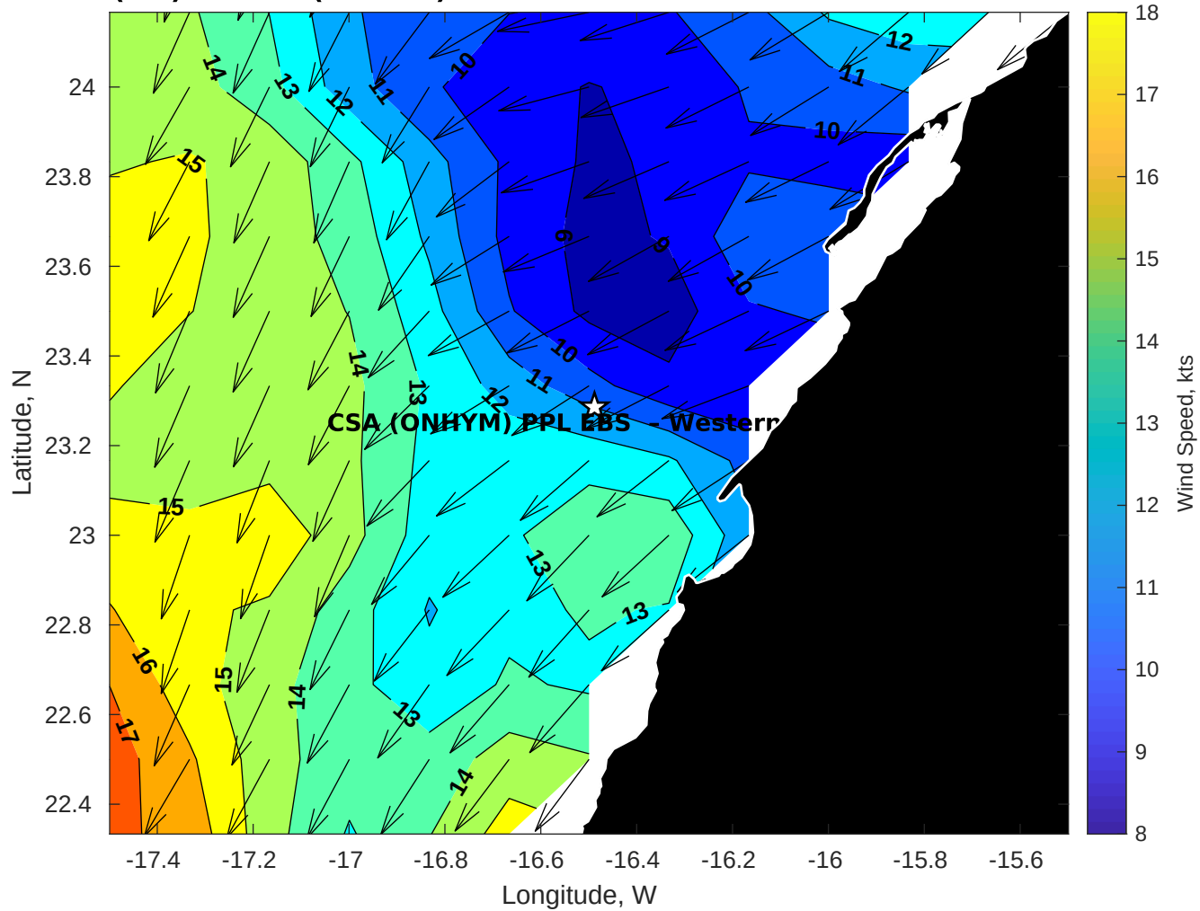
GFS Winds (kts) for CSA (ONHYM) PPL EBS - Western Sahara at 03-Feb-2026 09:00:00
