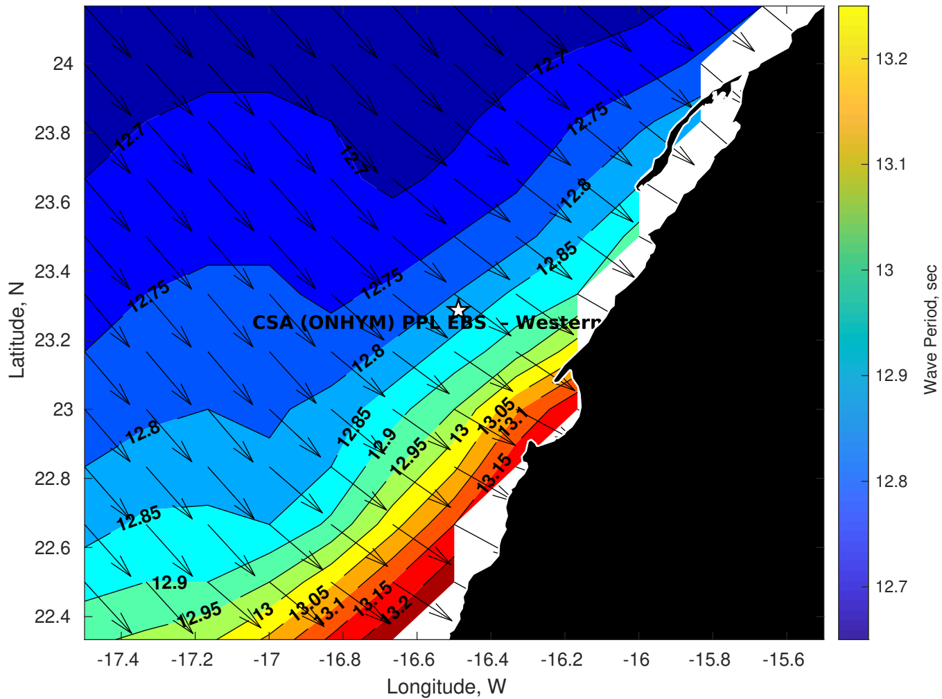
GFS Wave Period (sec) for CSA (ONHYM) PPL EBS - Western Sahara at 03-Feb-2026 09:00:00
