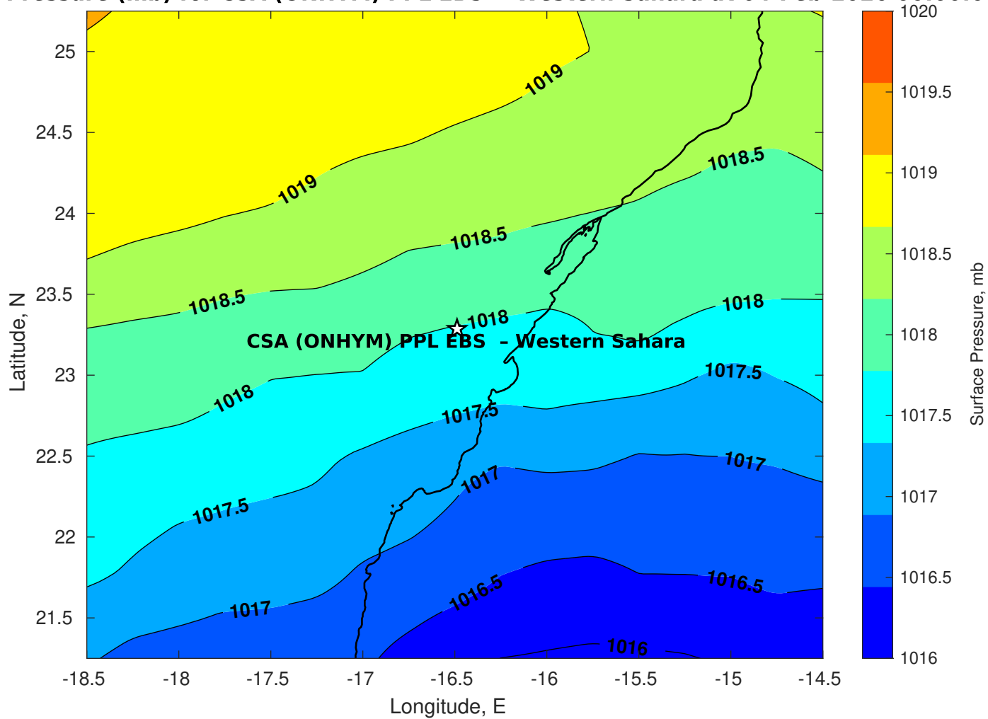
Surface Pressure (mb) for CSA (ONHYM) PPL EBS - Western Sahara at 04-Feb-2026 00:00:00
