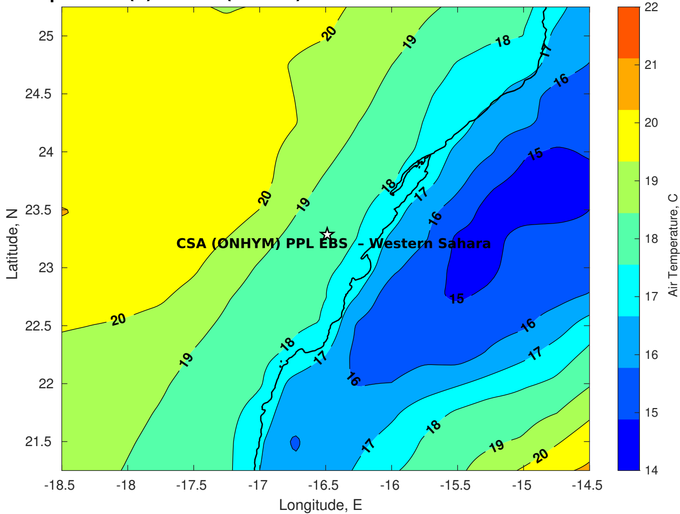
Air Temperature (C) for CSA (ONHYM) PPL EBS - Western Sahara at 03-Feb-2026
