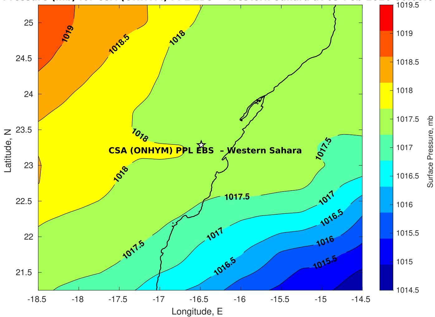
Surface Pressure (mb) for CSA (ONHYM) PPL EBS - Western Sahara at 03-Feb-2026 00:00:00
