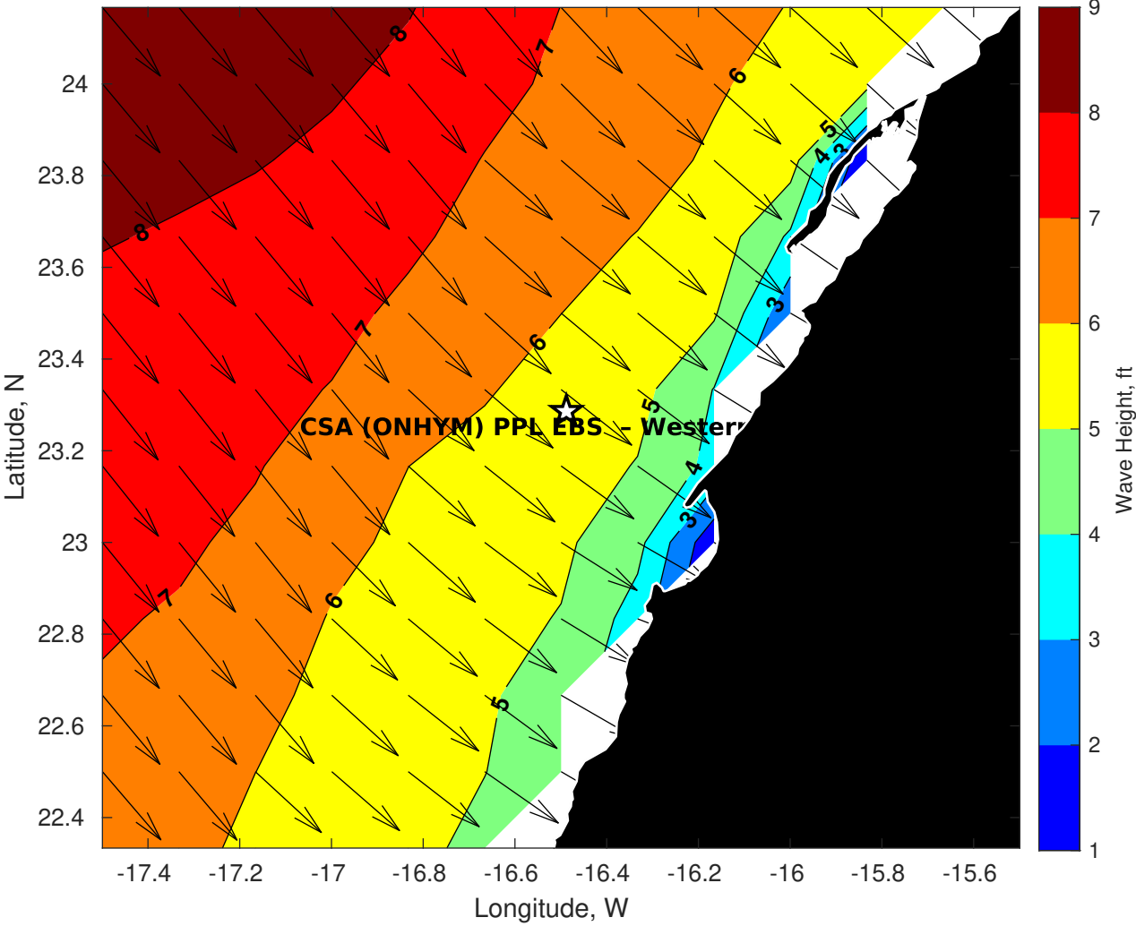
GFS Wave Height (ft) for CSA (ONHYM) PPL EBS - Western Sahara at 03-Feb-2026 09:00:00
