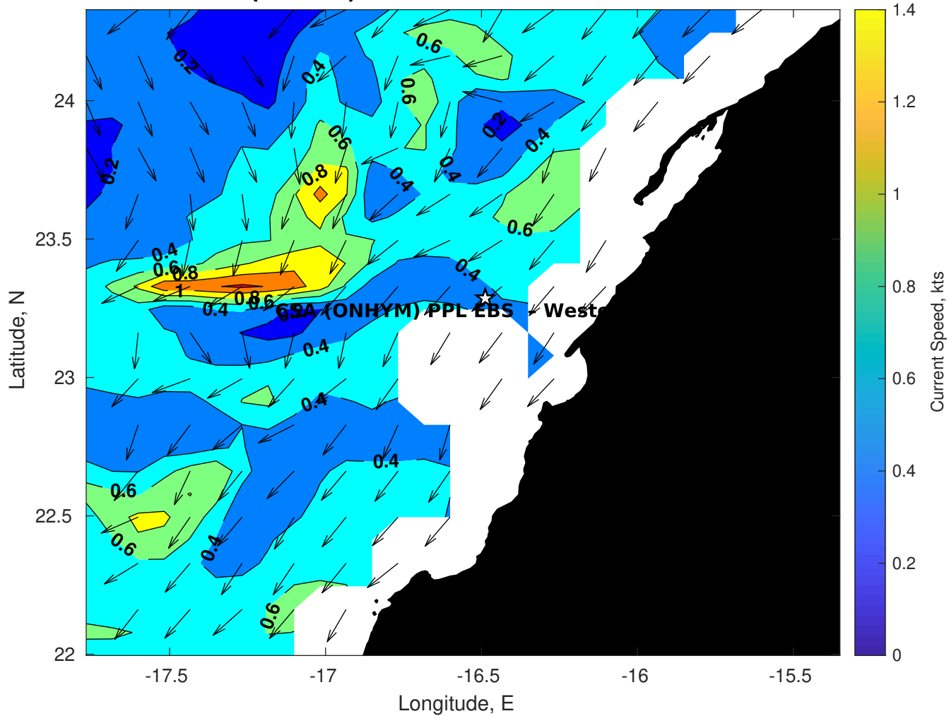
Surface Currents for CSA (ONHYM) PPL EBS - Western Sahara at 02-Feb-2026 00:00:00
