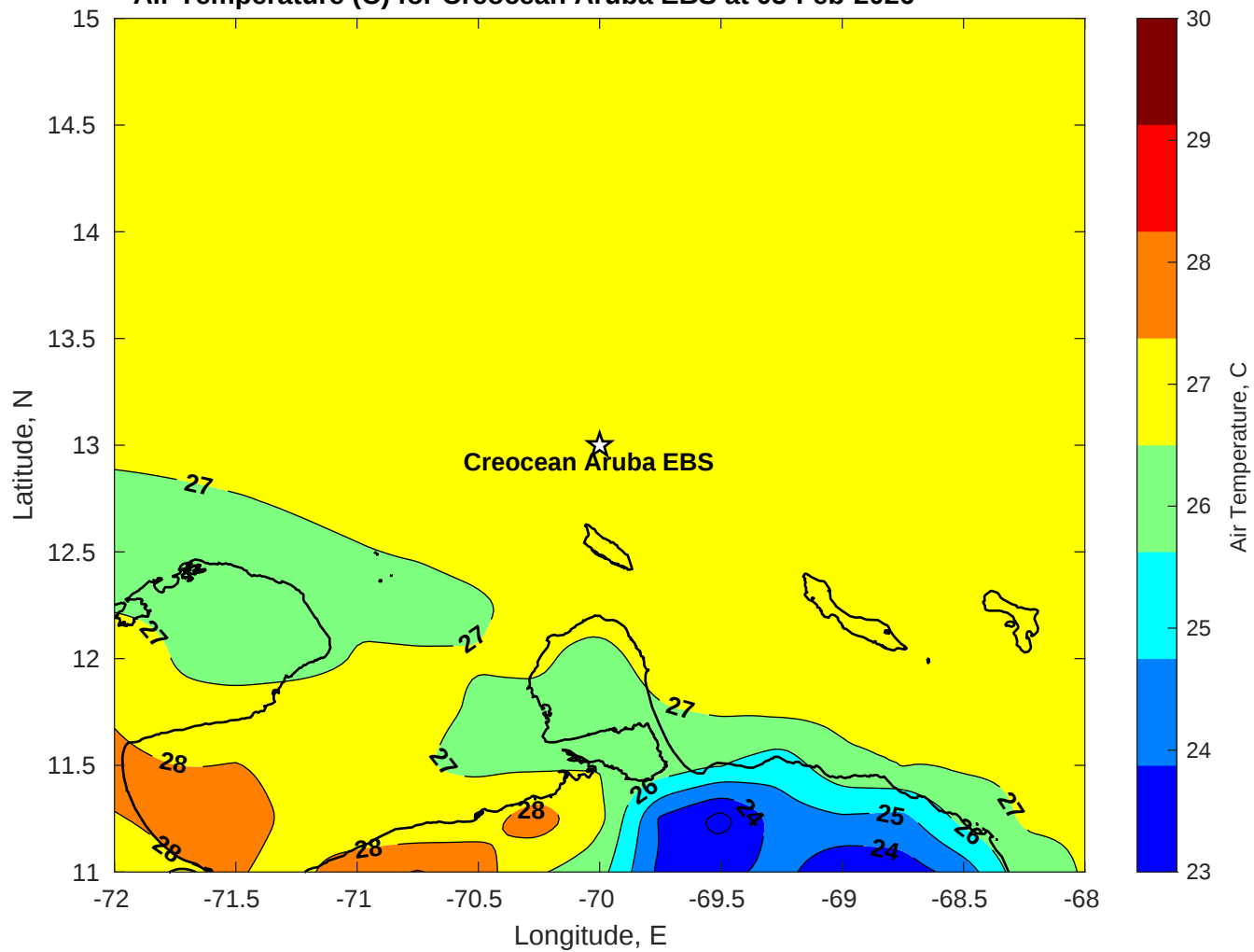
Air Temperature (C) for Creoccean Aruba EBS at 03-Feb-2026
