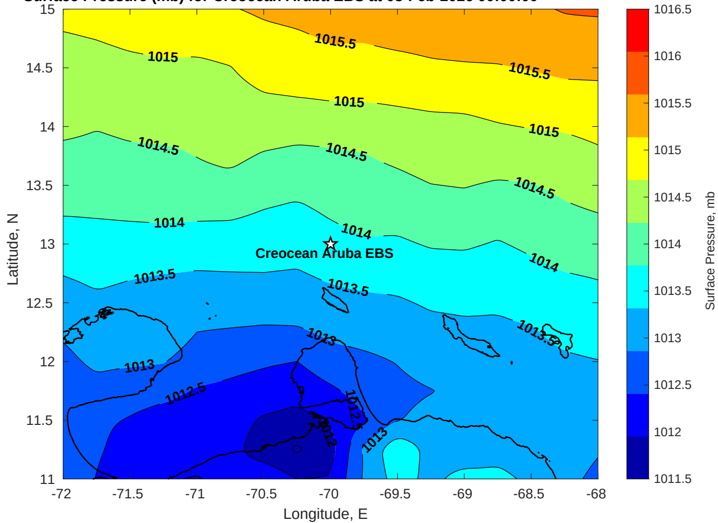
Surface Pressure (mb) for Creocean Aruba EBS at 03-Feb-2026 00:00:00
