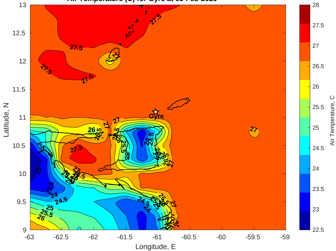
Air Temperature (C) for Gyre at 03-Feb-2026
