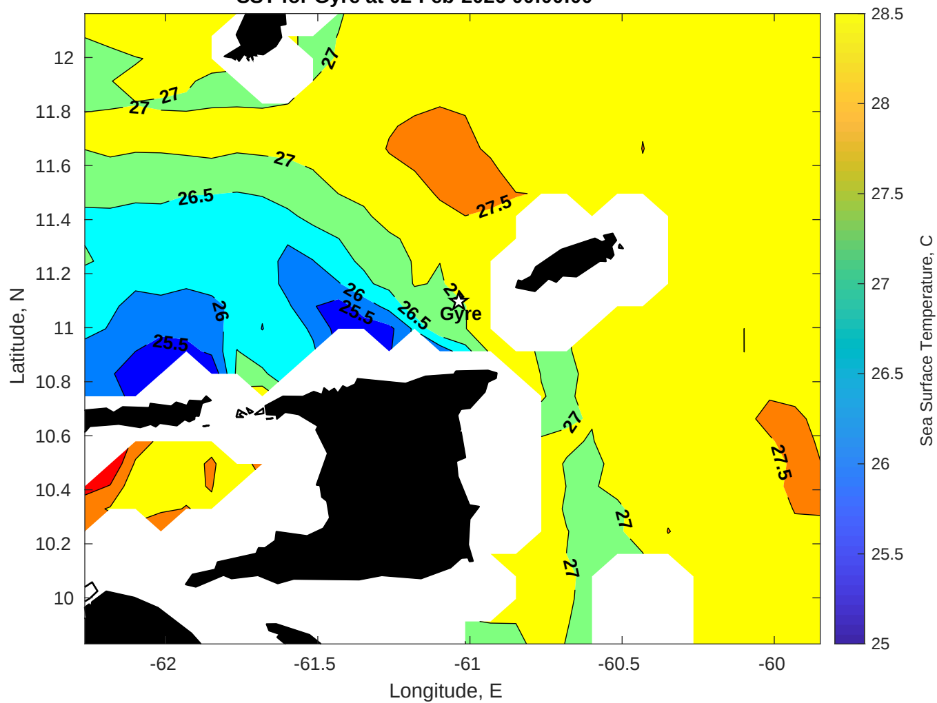
SST for Gyre at 02-Feb-2026 00:00:00
