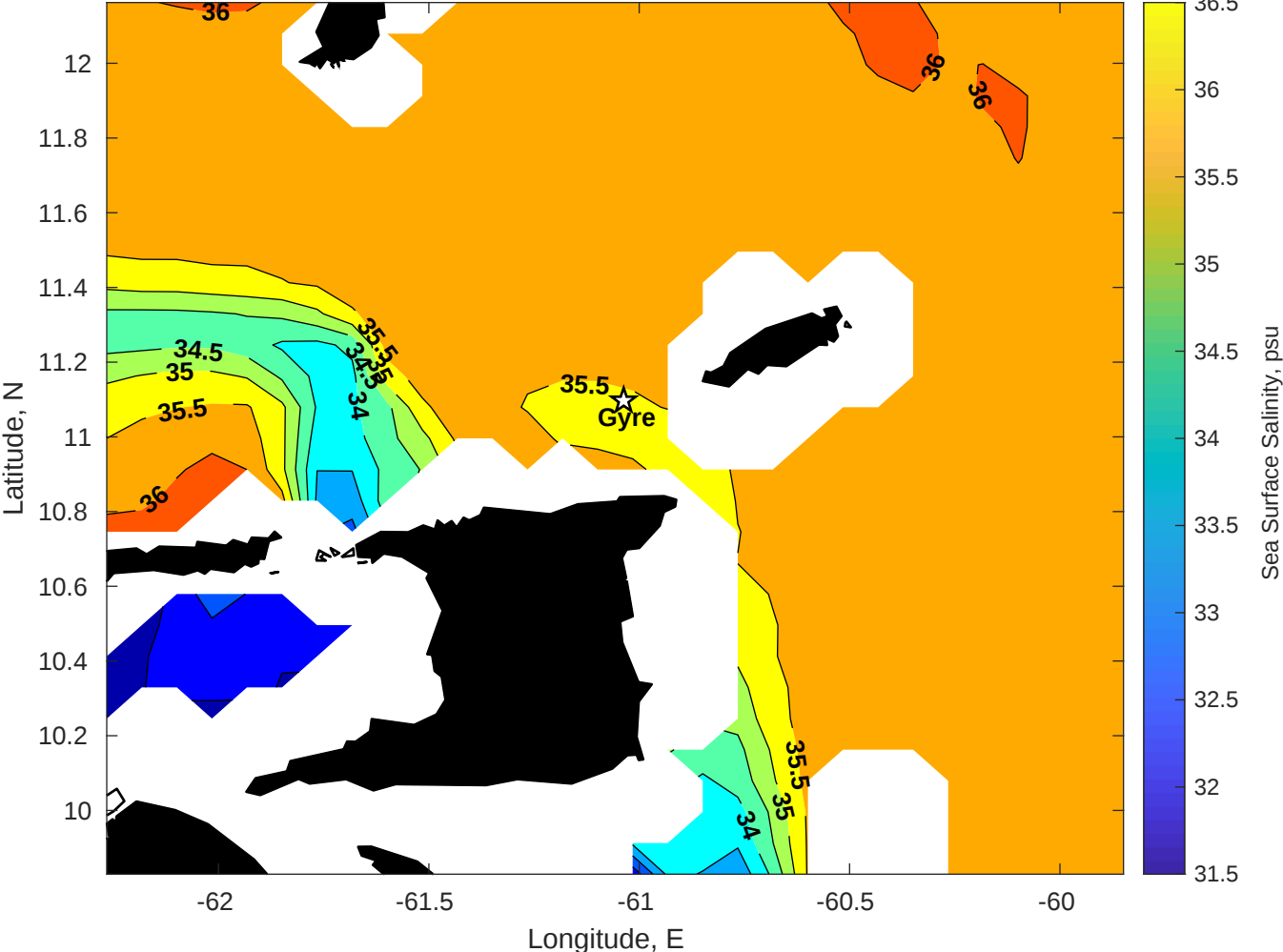
Surface Salinity for Gyre at 02-Feb-2026 00:00:00
