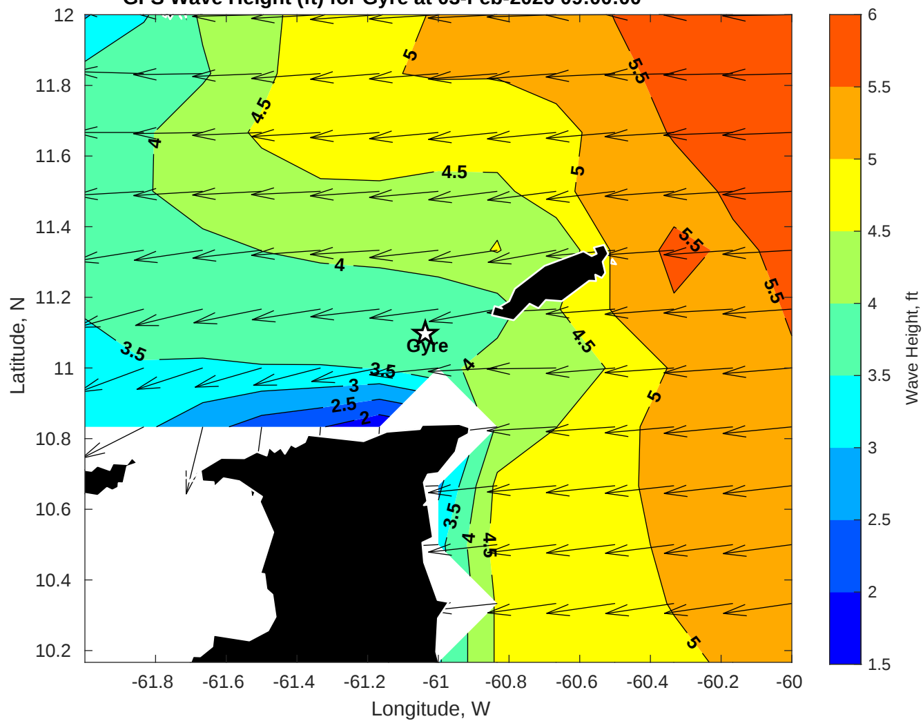
GFS Wave Height (ft) for Gyre at 03-Feb-2026 09:00:00
