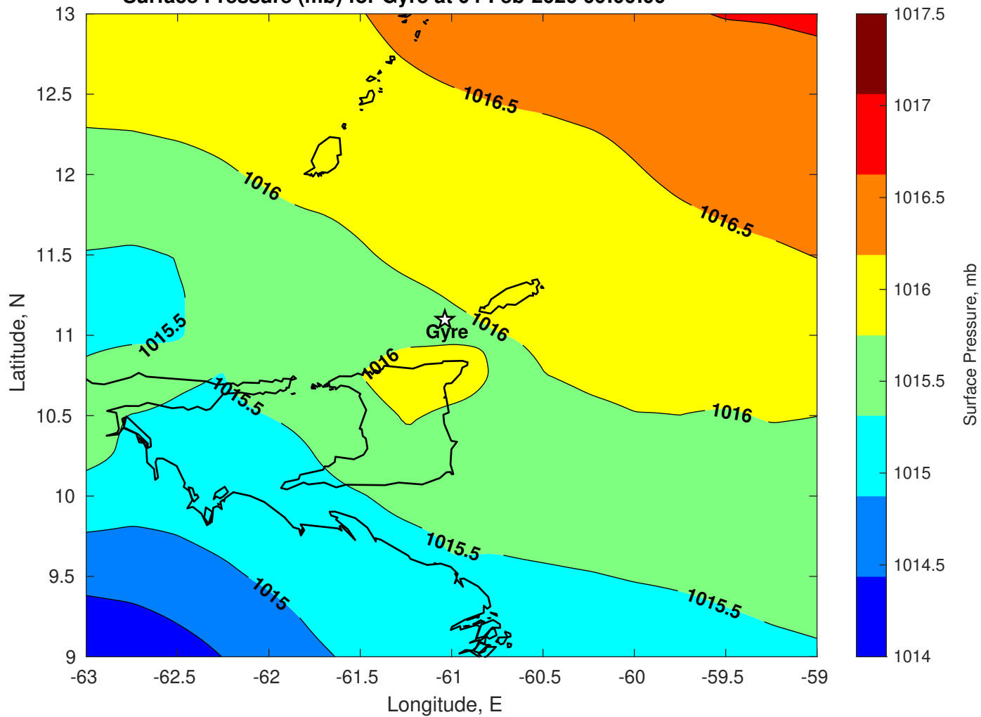
Surface Pressure (mb) for Gyre at 04-Feb-2026 00:00:00
