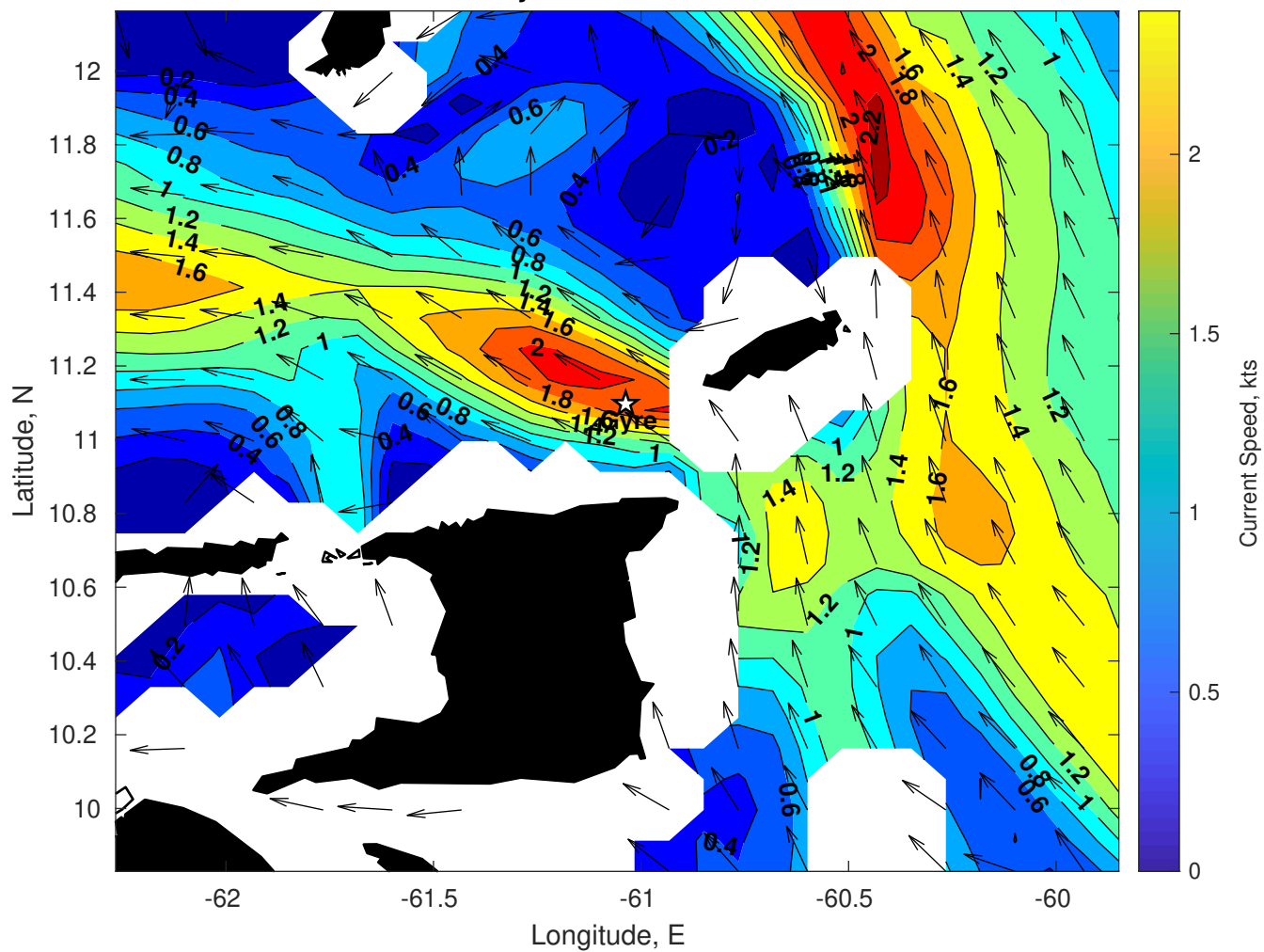
Surface Currents for Gyre at 02-Feb-2026 00:00:00
