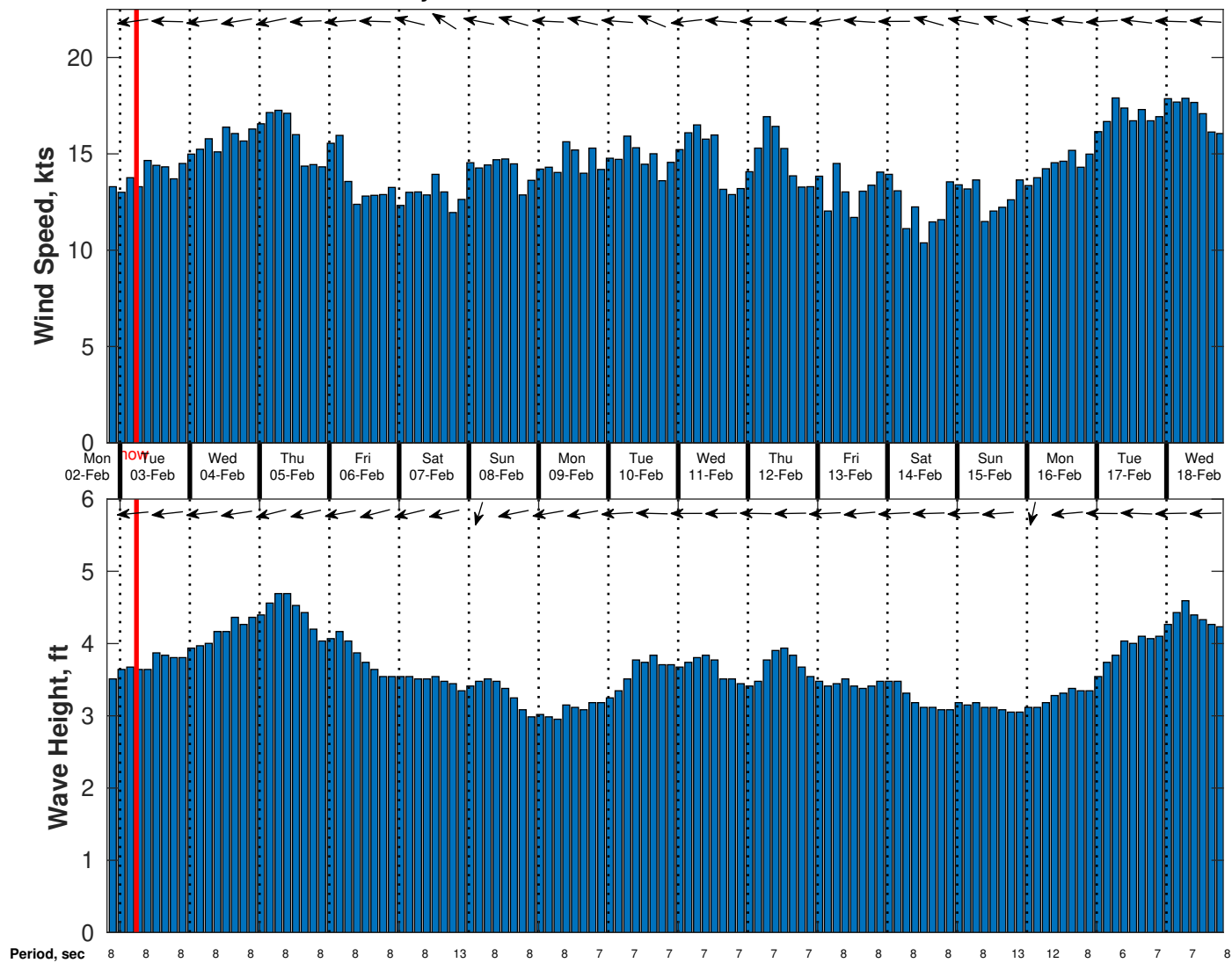
Wind & Wave Forecast for Gyre from 02-Feb-2026 20:00:00 to 18-Feb-2026 20:00:00
