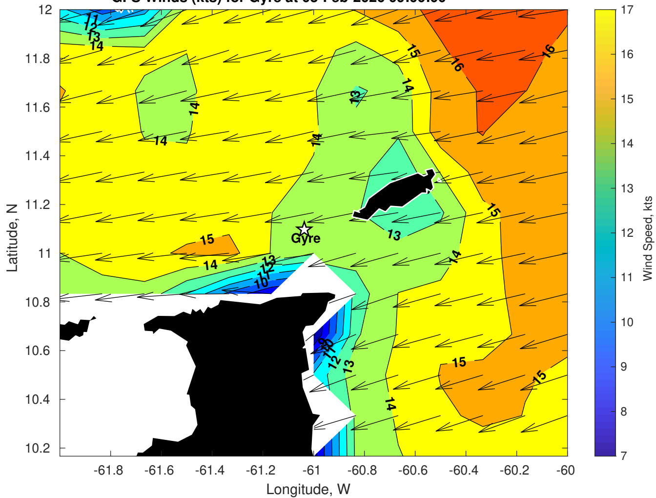
GFS Winds (kts) for Gyre at 03-Feb-2026 09:00:00
