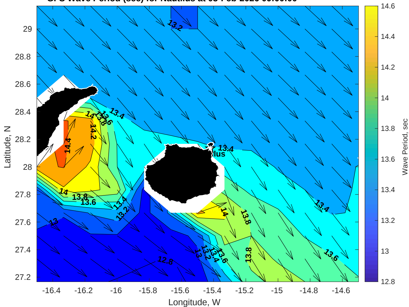
GFS Wave Period (sec) for Nautilus at 03-Feb-2026 09:00:00
