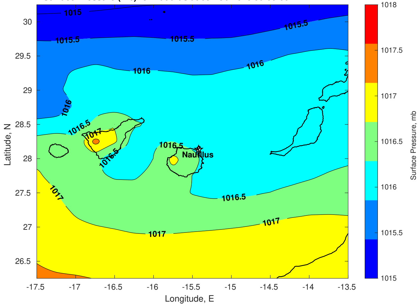
Surface Pressure (mb) for Nautilus at 05-Feb-2026 00:00:00
