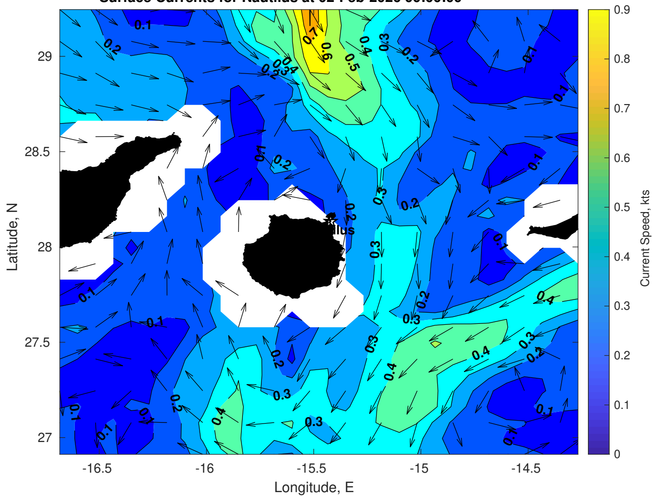
Surface Currents for Nautilus at 02-Feb-2026 00:00:00
