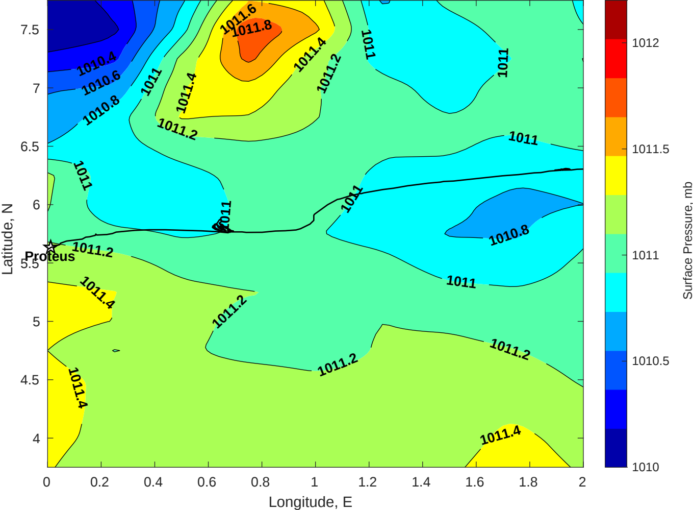
Surface Pressure (mb) for Proteus at 03-Feb-2026 00:00:00
