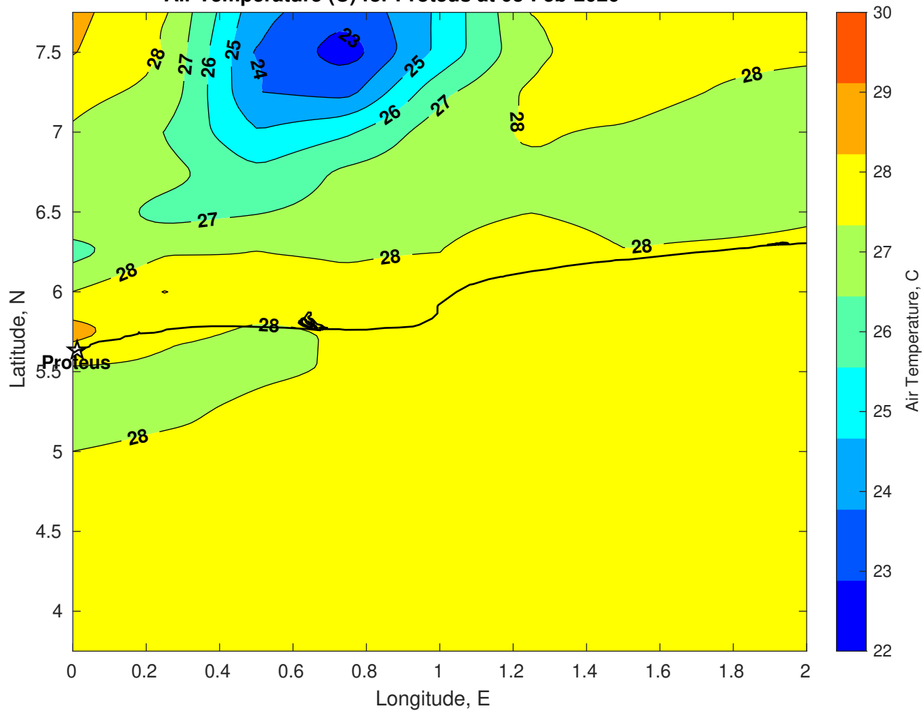
Air Temperature (C) for Proteus at 03-Feb-2026
