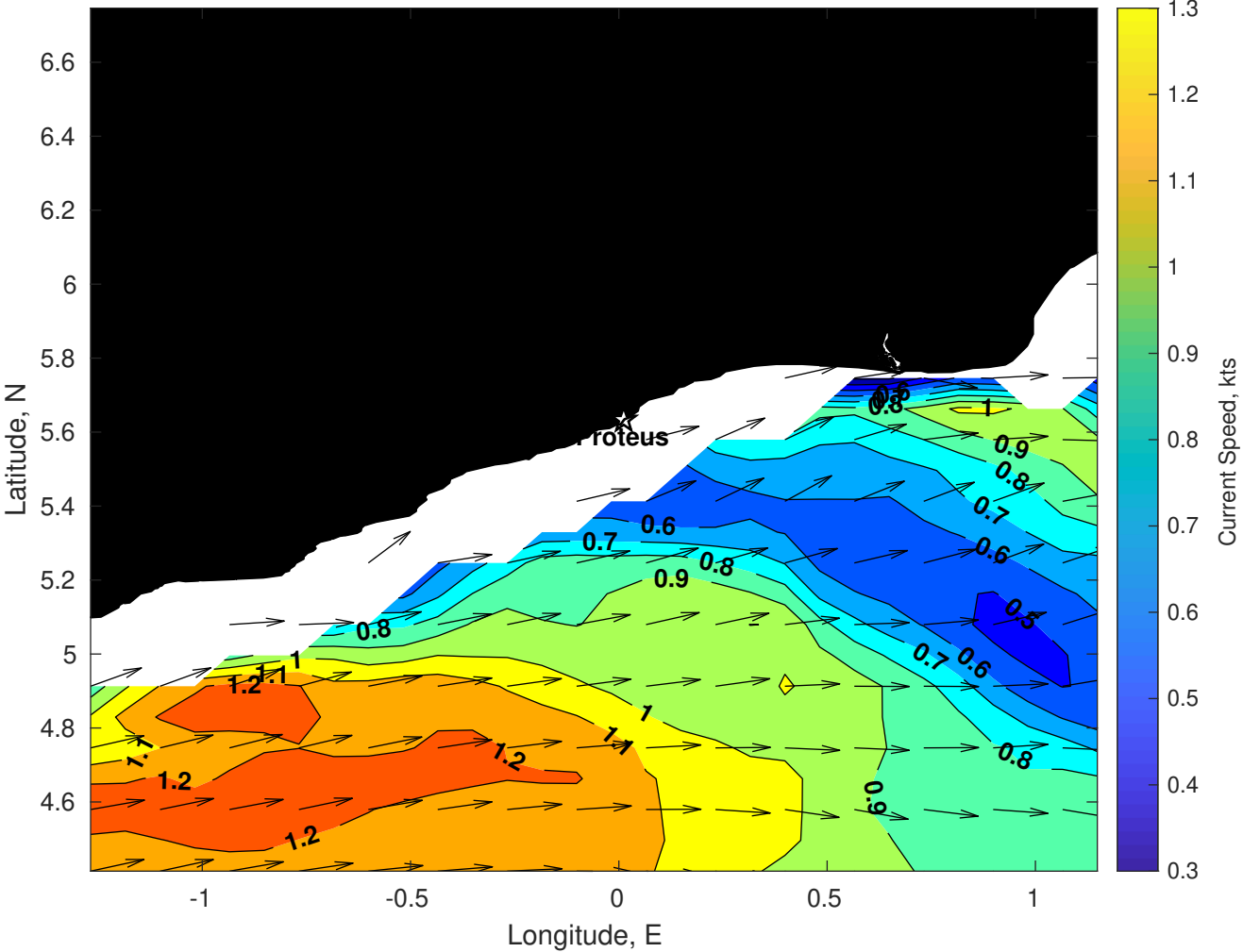
Surface Currents for Proteus at 02-Feb-2026 00:00:00
