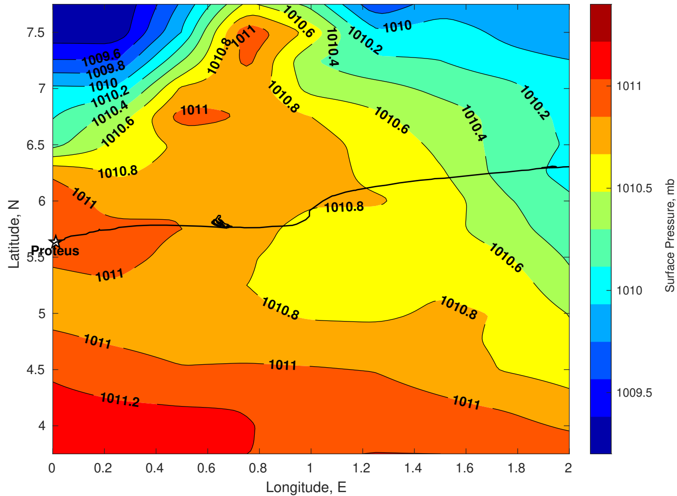
Surface Pressure (mb) for Proteus at 05-Feb-2026 00:00:00
