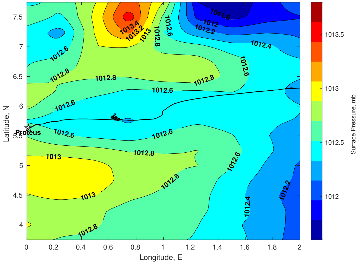
Surface Pressure (mb) for Proteus at 04-Feb-2026 00:00:00
