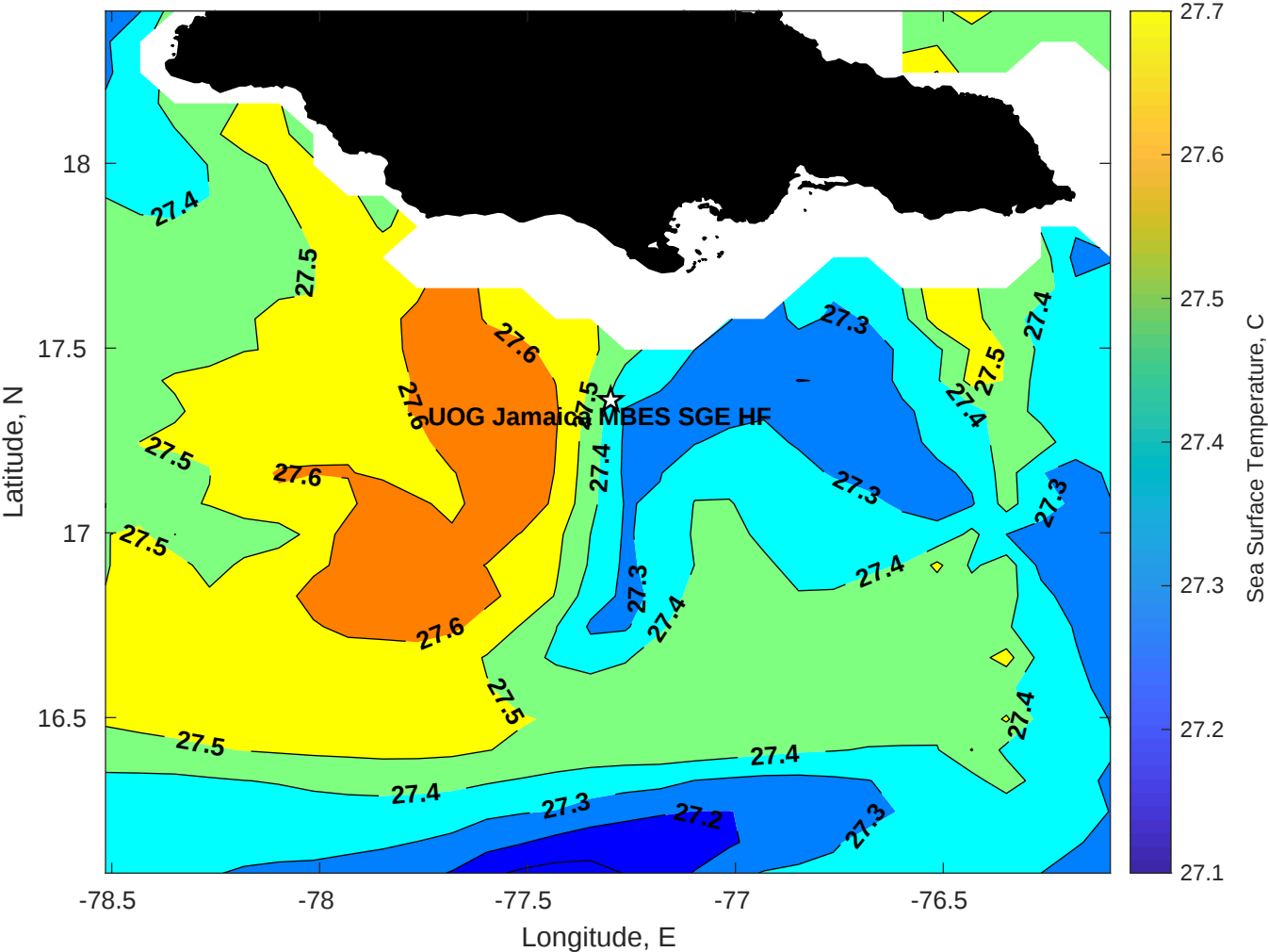
SST for UOG Jamaica MBES SGE HF at 02-Feb-2026 00:00:00
