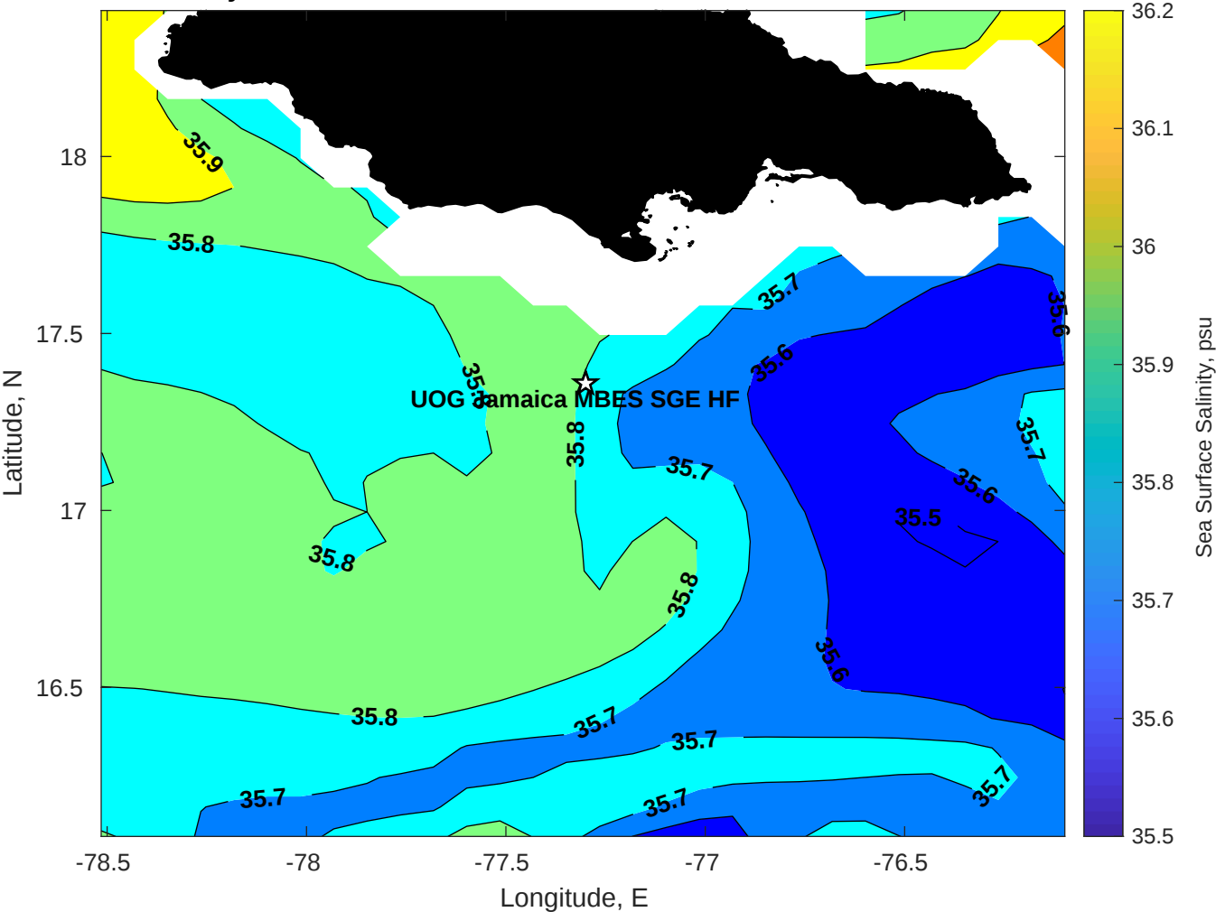
Surface Salinity for UOG Jamaica MBES SGE HF at 02-Feb-2026 00:00:00
