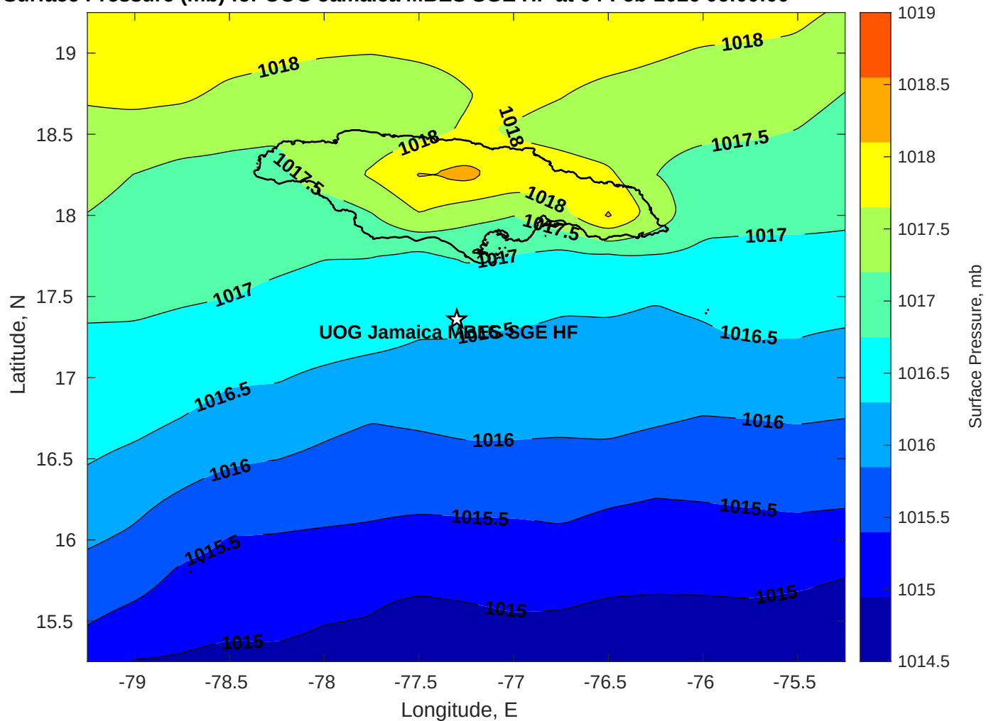
Surface Pressure (mb) for UOG Jamaica MBES SGE HF at 04-Feb-2026 06:00:00
