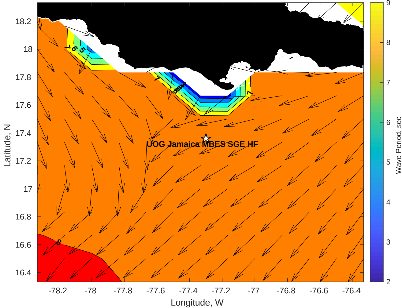
GFS Wave Period (sec) for UOG Jamaica MBES SGE HF at 03-Feb-2026 09:00:00
