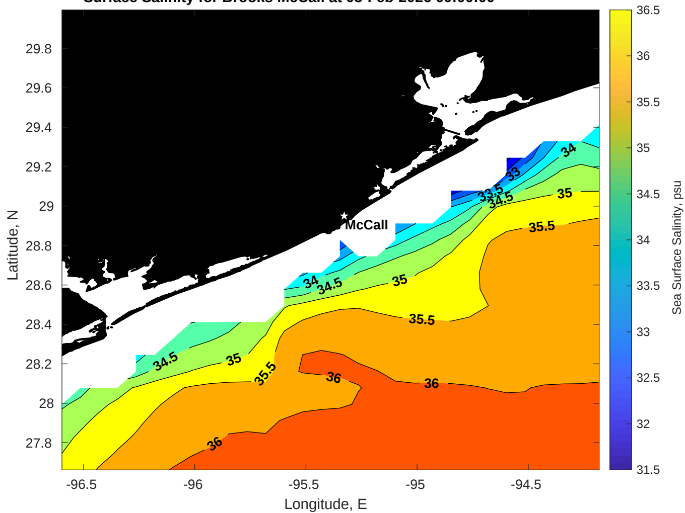
Surface Salinity for Brooks McCall at 03-Feb-2026 00:00:00
