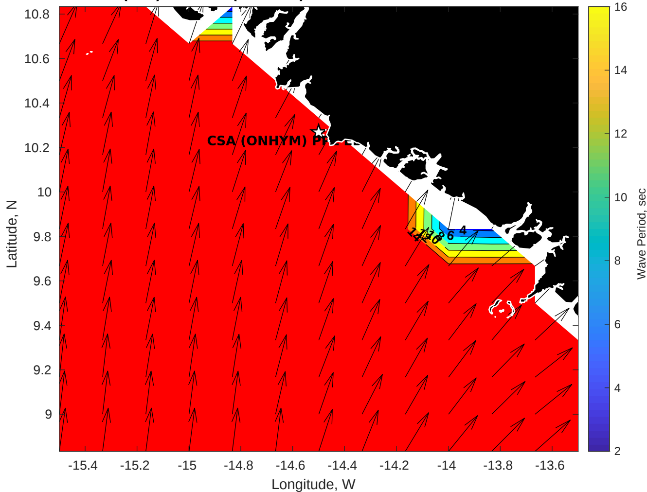
GFS Wave Period (sec) for CSA (ONHYM) PPL EBS - Guinea at 04-Feb-2026 09:00:00
