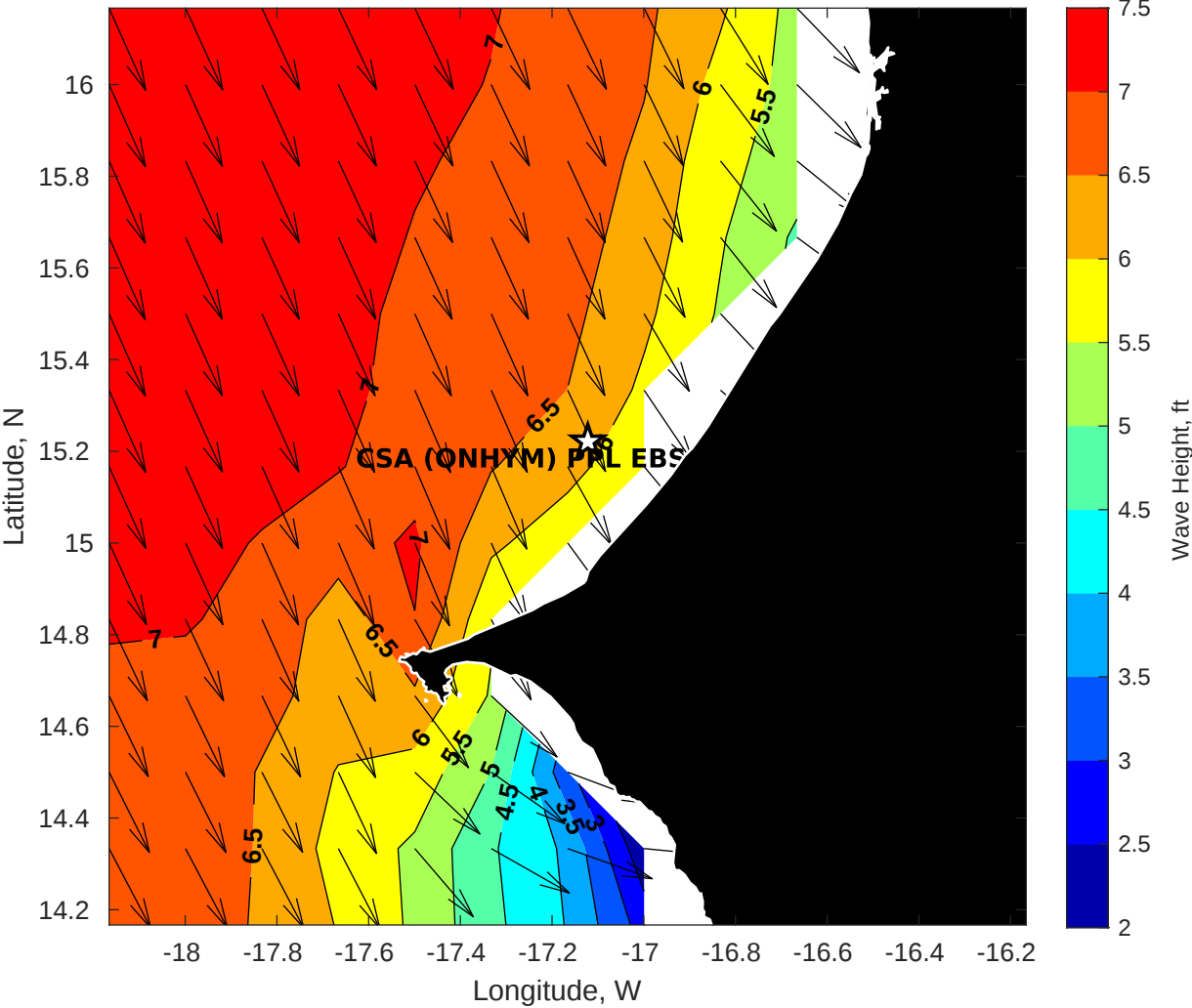
GFS Wave Height (ft) for CSA (ONHYM) PPL EBS - Senegal at 04-Feb-2026 09:00:00
