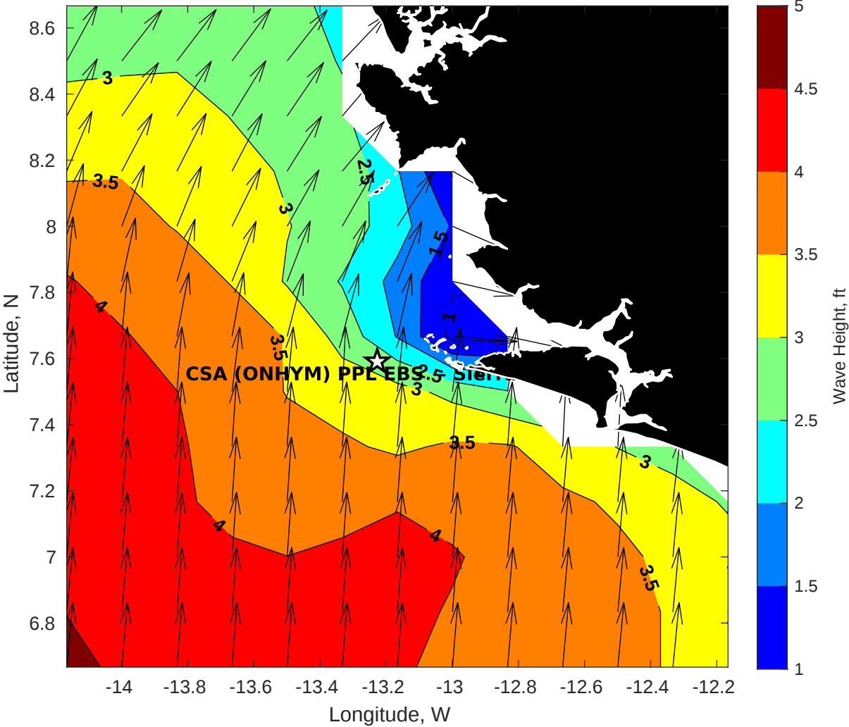
GFS Wave Height (ft) for CSA (ONHYM) PPL EBS - Sierra Leone at 04-Feb-2026 09:00:00
