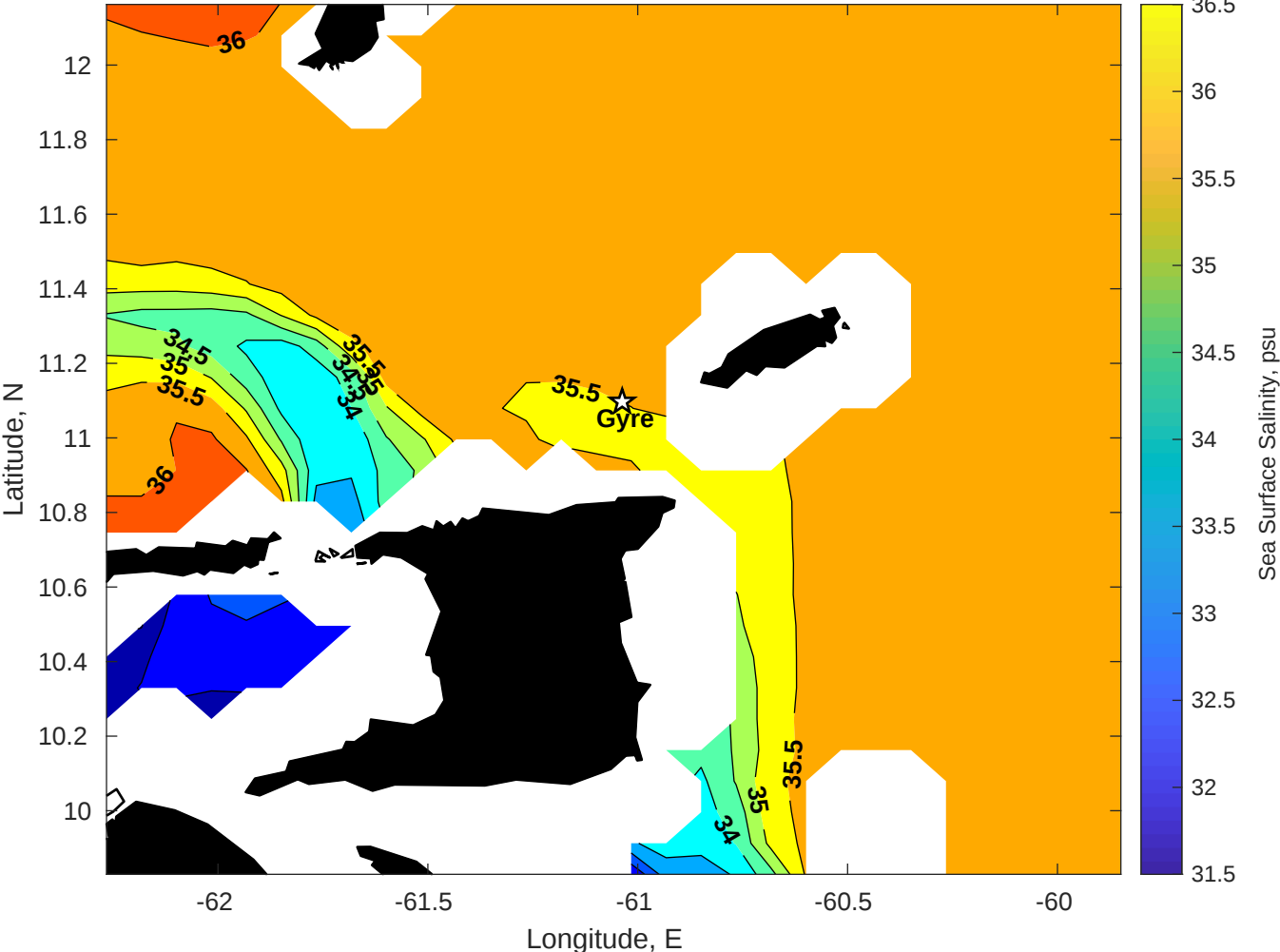
Surface Salinity for Gyre at 03-Feb-2026 00:00:00
