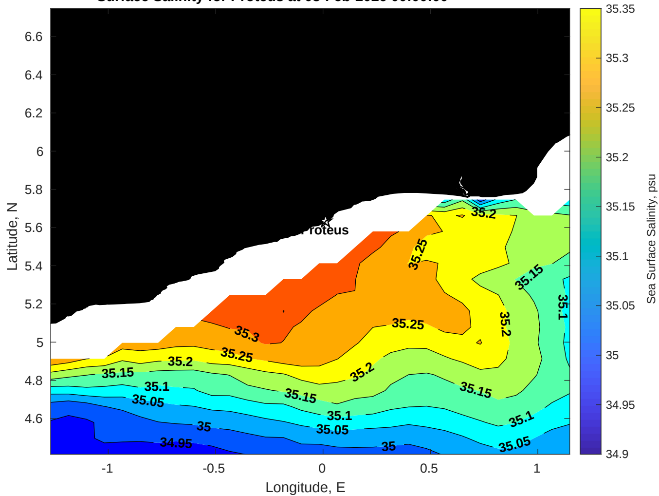
Surface Salinity for Proteus at 03-Feb-2026 00:00:00
