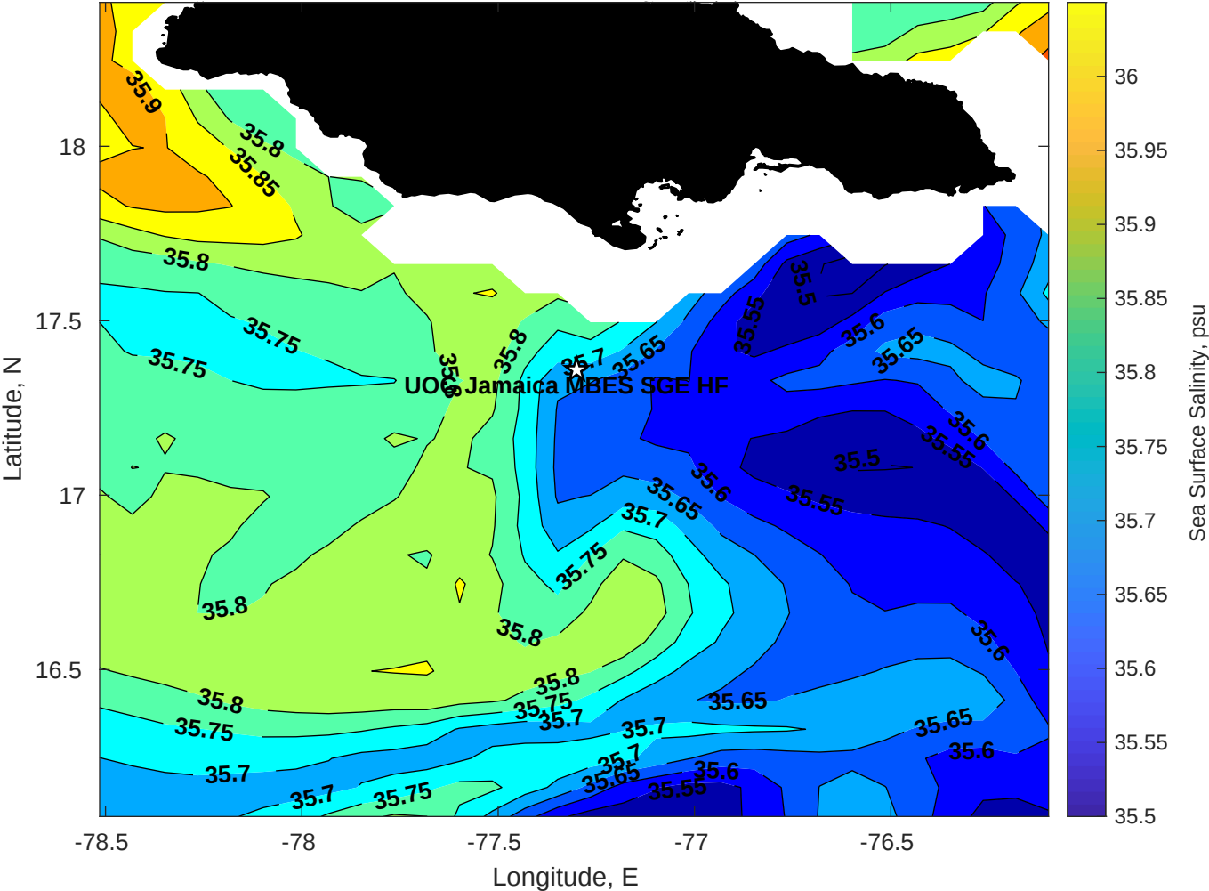
Surface Salinity for UOG Jamaica MBES SGE HF at 03-Feb-2026 00:00:00
