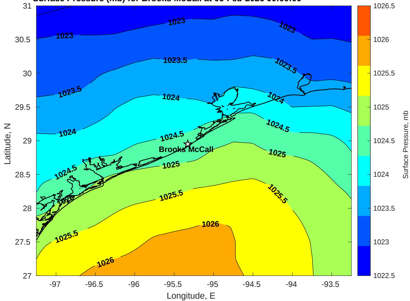
Surface Pressure (mb) for Brooks McCall at 06-Feb-2026 00:00:00
