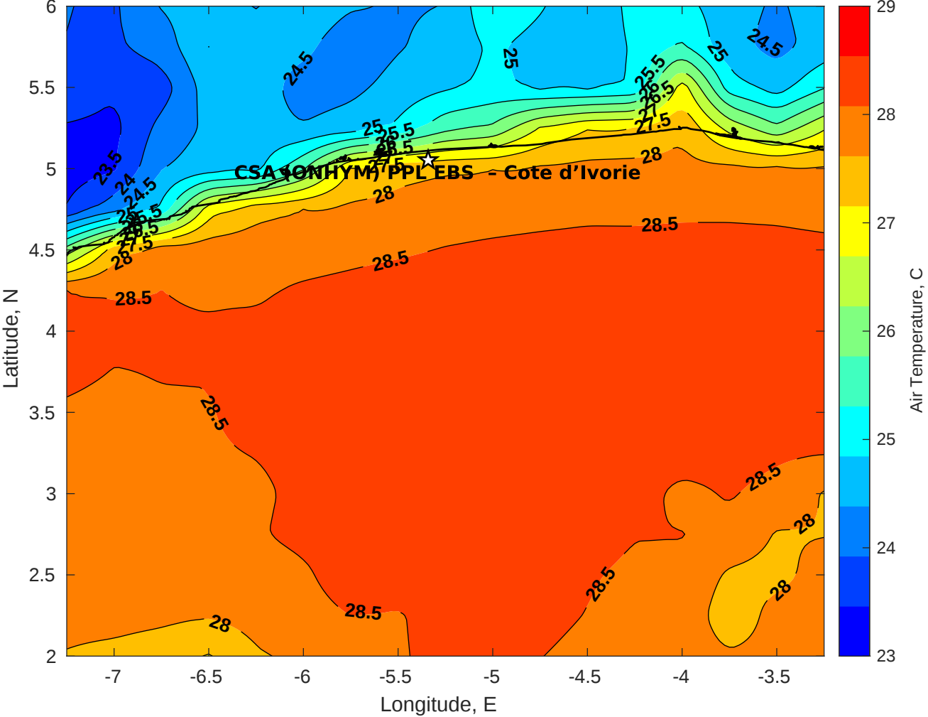
Air Temperature (C) for CSA (ONHYM) PPL EBS - Cote d'Ivoire at 05-Feb-2026
