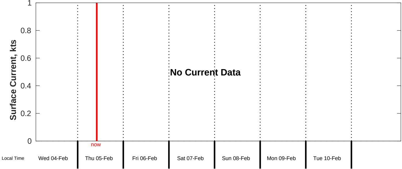
Surface Current Forecast for CSA (ONHYM) PPL EBS - Cote d'Ivoire from 04-Feb-2026 00:00:00 to 12-Feb-2026 00:00:00
