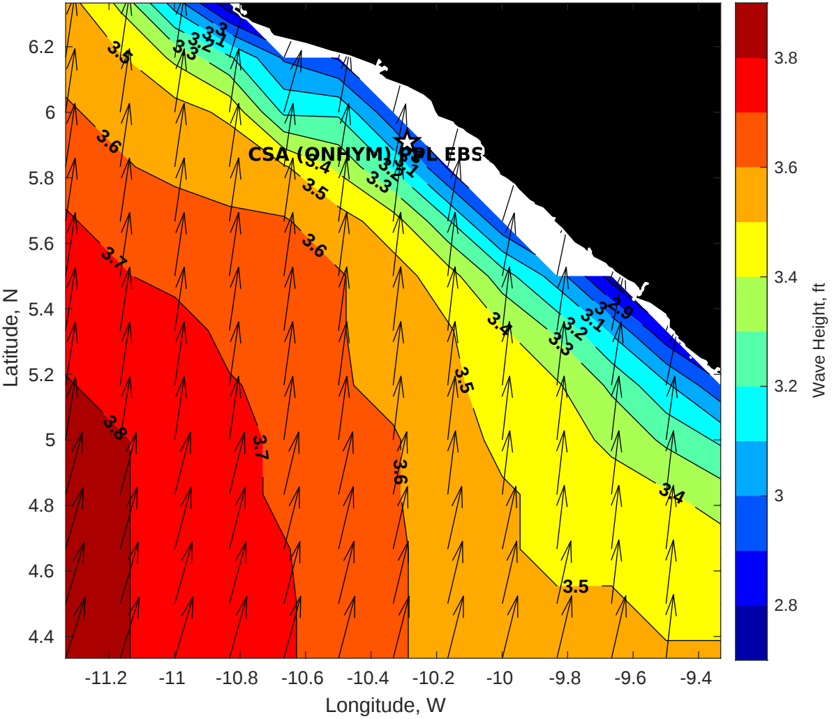
GFS Wave Height (ft) for CSA (ONHYM) PPL EBS - Liberia at 05-Feb-2026 09:00:00
