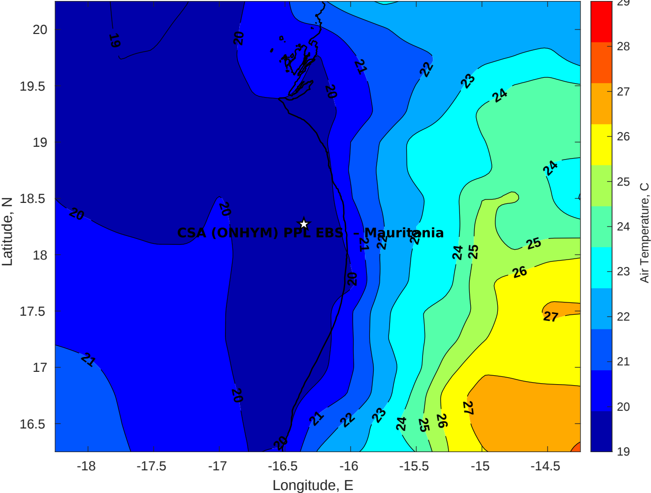
Air Temperature (C) for CSA (ONHYM) PPL EBS - Mauritania at 05-Feb-2026
