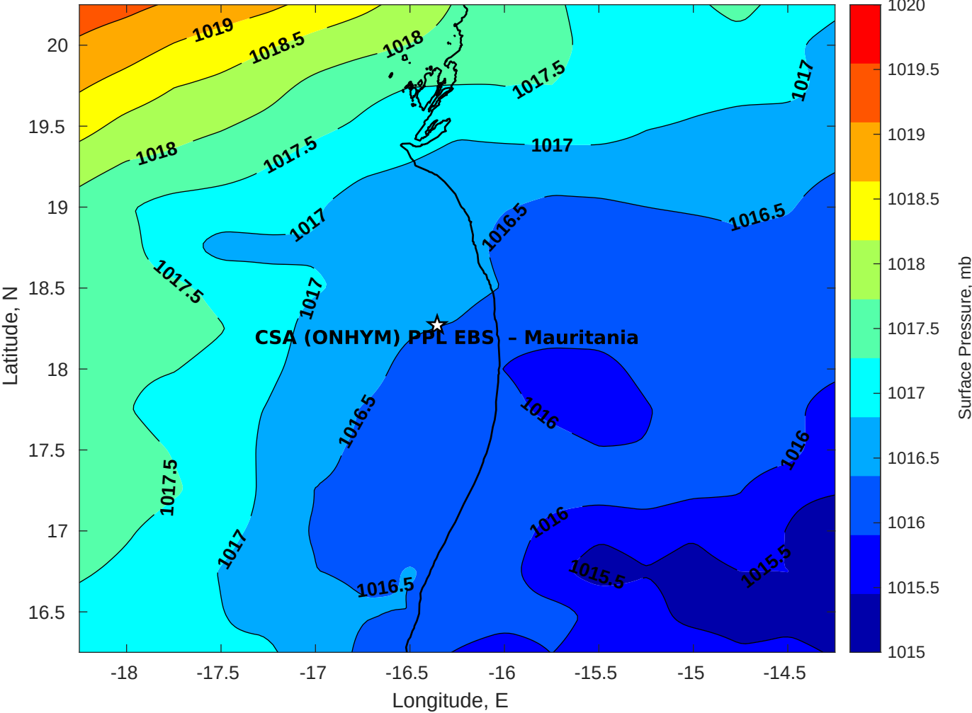
Surface Pressure (mb) for CSA (ONHYM) PPL EBS - Mauritania at 07-Feb-2026 00:00:00
