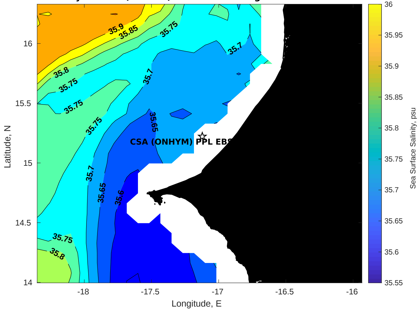
Surface Salinity for CSA (ONHYM) PPL EBS - Senegal at 04-Feb-2026 00:00:00
