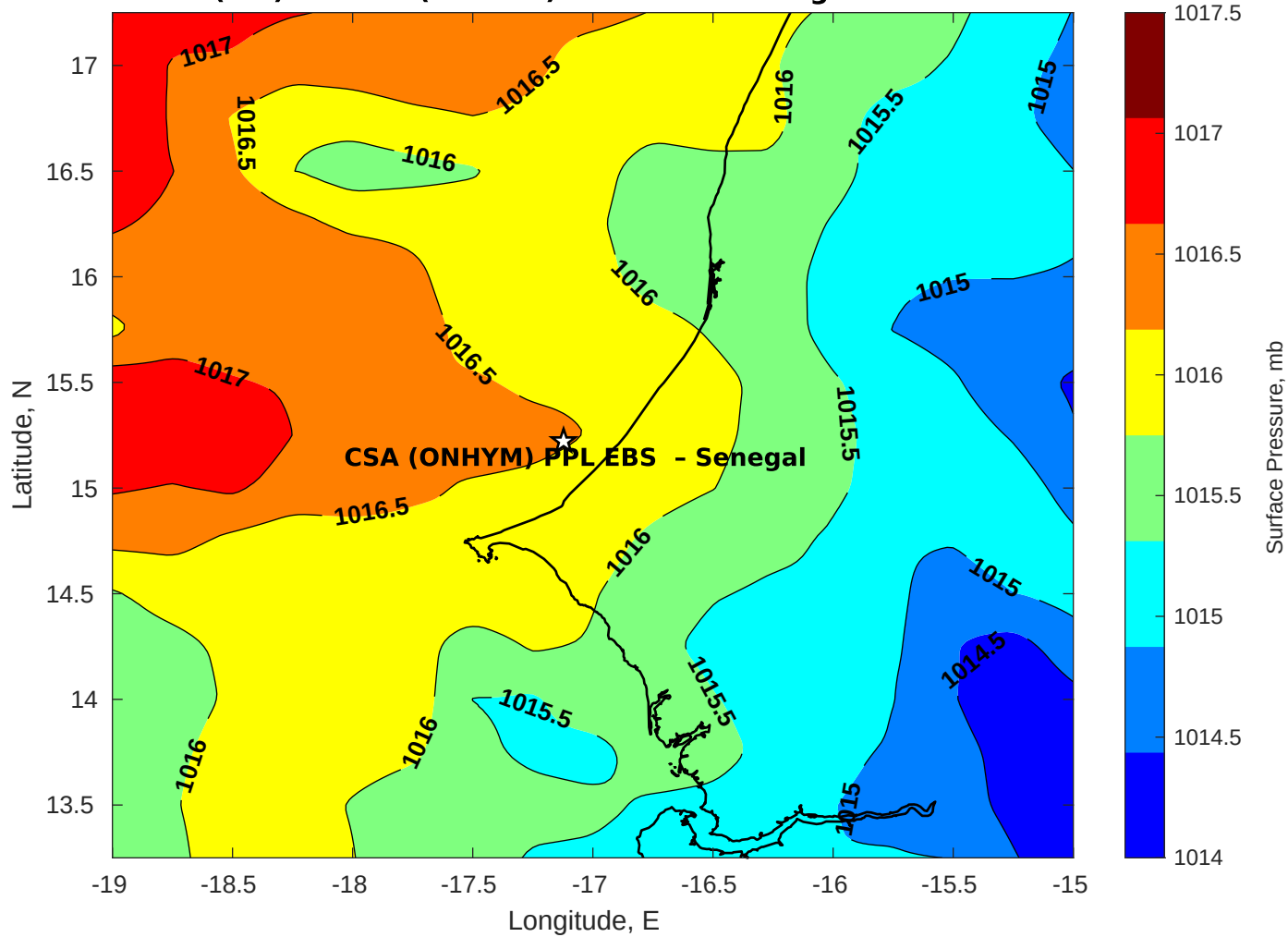
Surface Pressure (mb) for CSA (ONHYM) PPL EBS - Senegal at 06-Feb-2026 00:00:00
