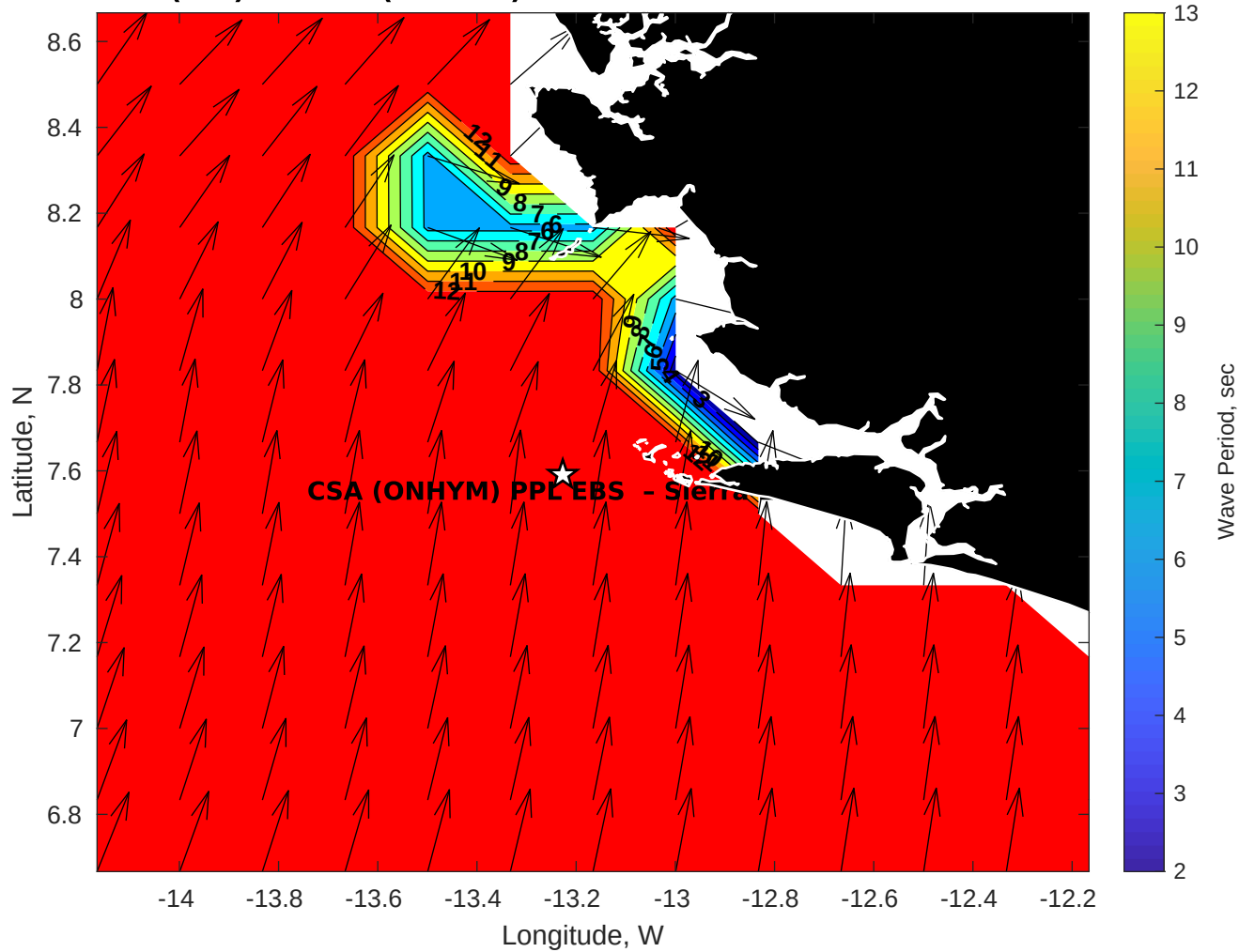
GFS Wave Period (sec) for CSA (ONHYM) PPL EBS - Sierra Leone at 05-Feb-2026 09:00:00
