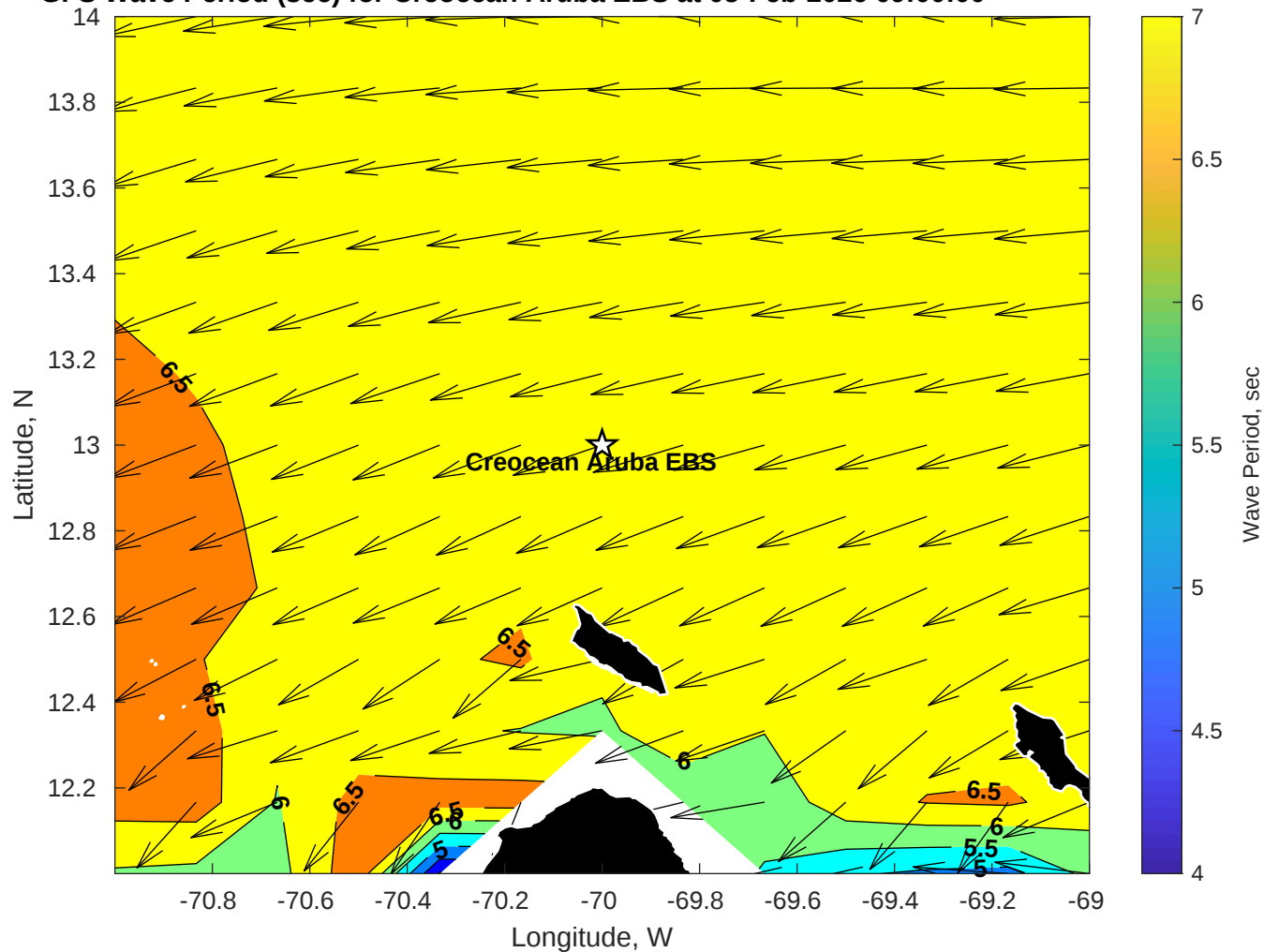
GFS Wave Period (sec) for Creoccean Aruba EBS at 05-Feb-2026 09:00:00
