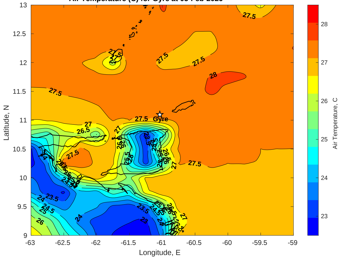
Air Temperature (C) for Gyre at 05-Feb-2026
