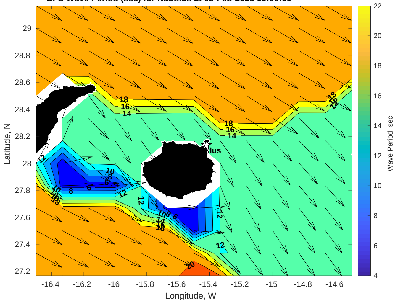
GFS Wave Period (sec) for Nautilus at 05-Feb-2026 09:00:00
