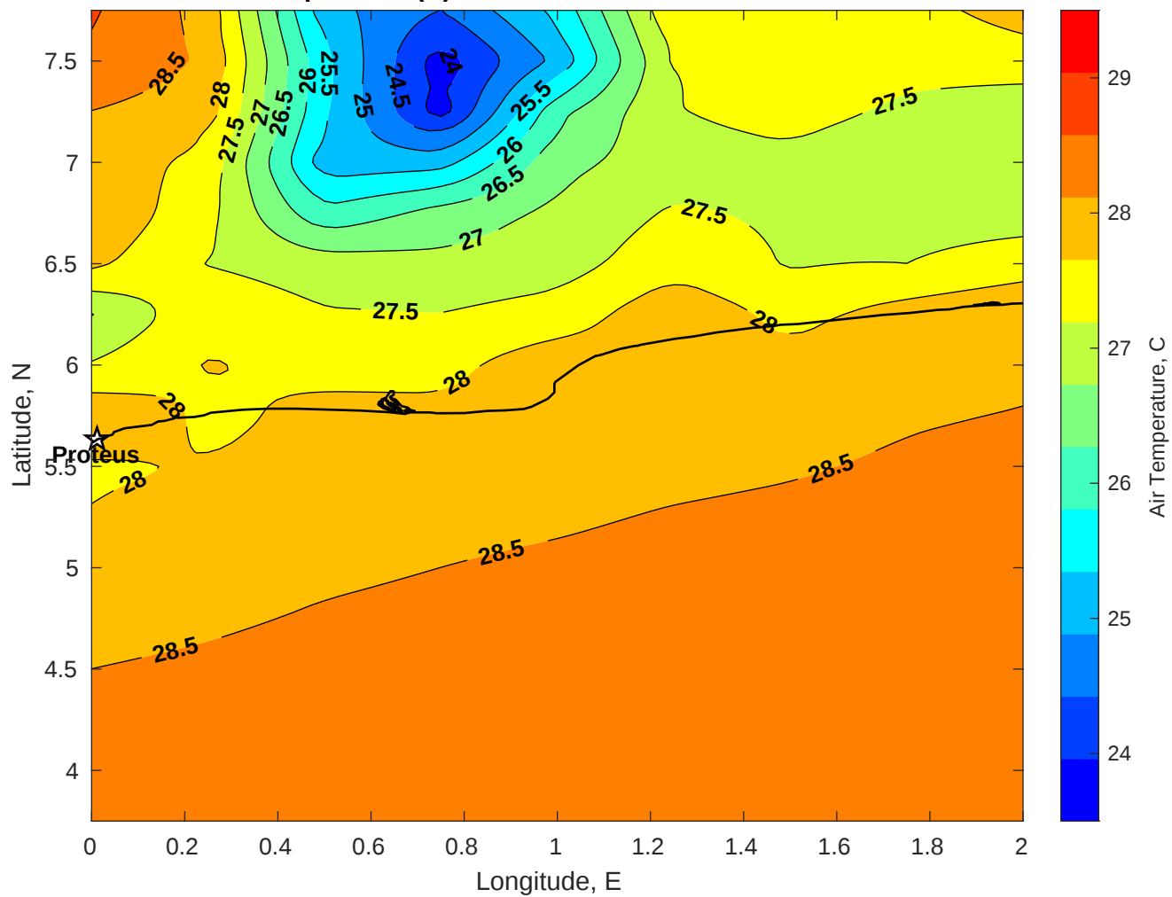
Air Temperature (C) for Proteus at 05-Feb-2026
