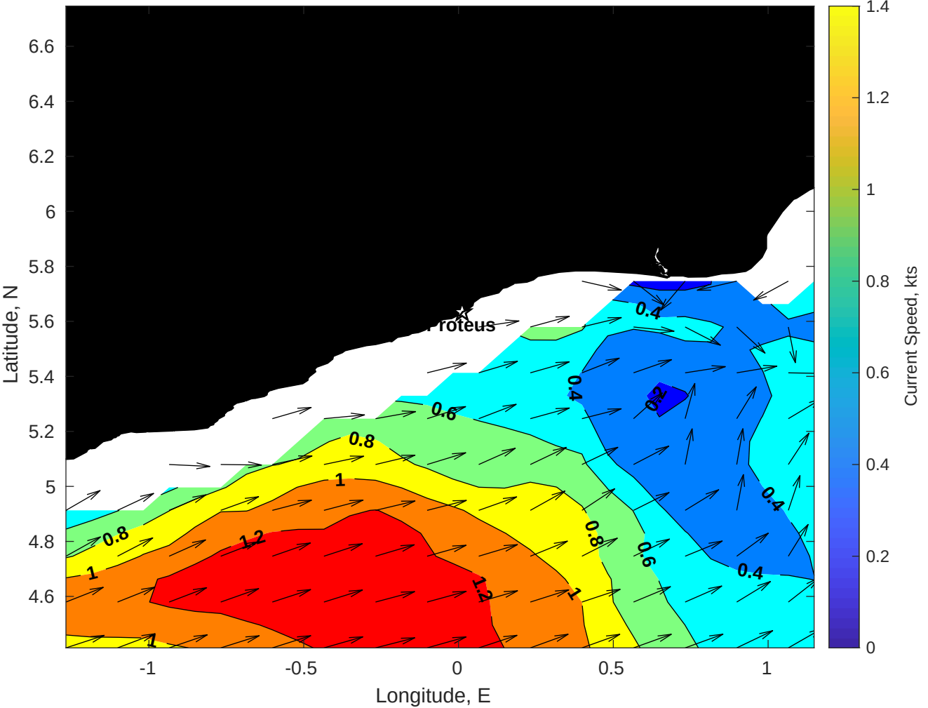
Surface Currents for Proteus at 04-Feb-2026 00:00:00
