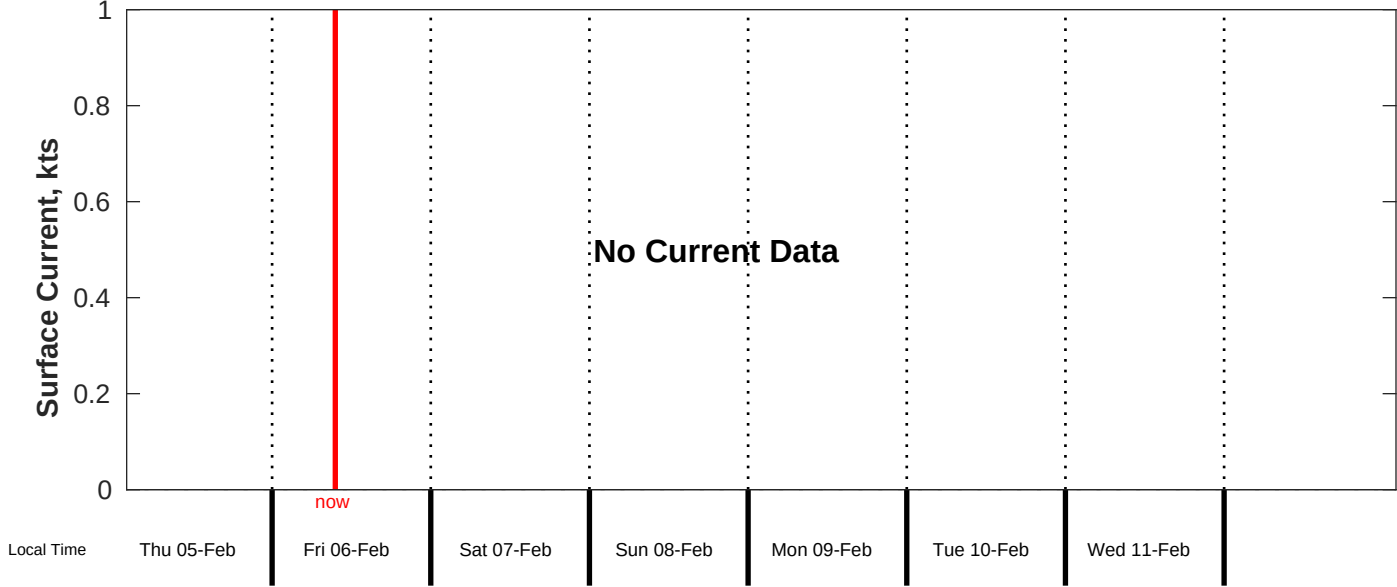
Surface Current Forecast for CSA (ONHYM) PPL EBS - Guinea from 05-Feb-2026 00:00:00 to 13-Feb-2026 00:00:00
