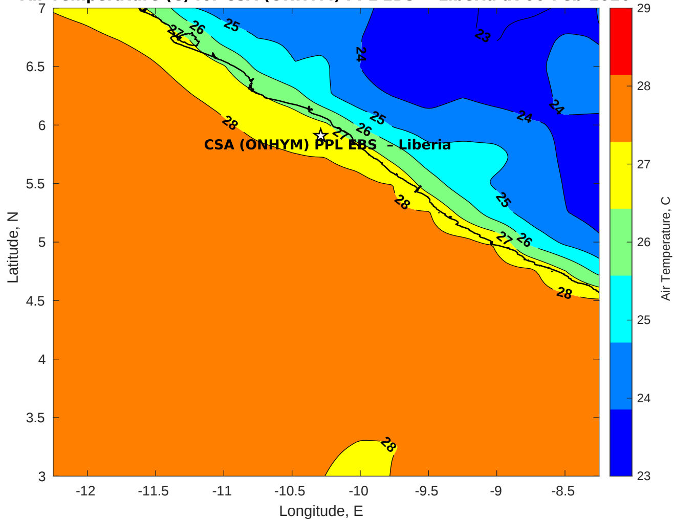
Air Temperature (C) for CSA (ONHYM) PPL EBS - Liberia at 06-Feb-2026
