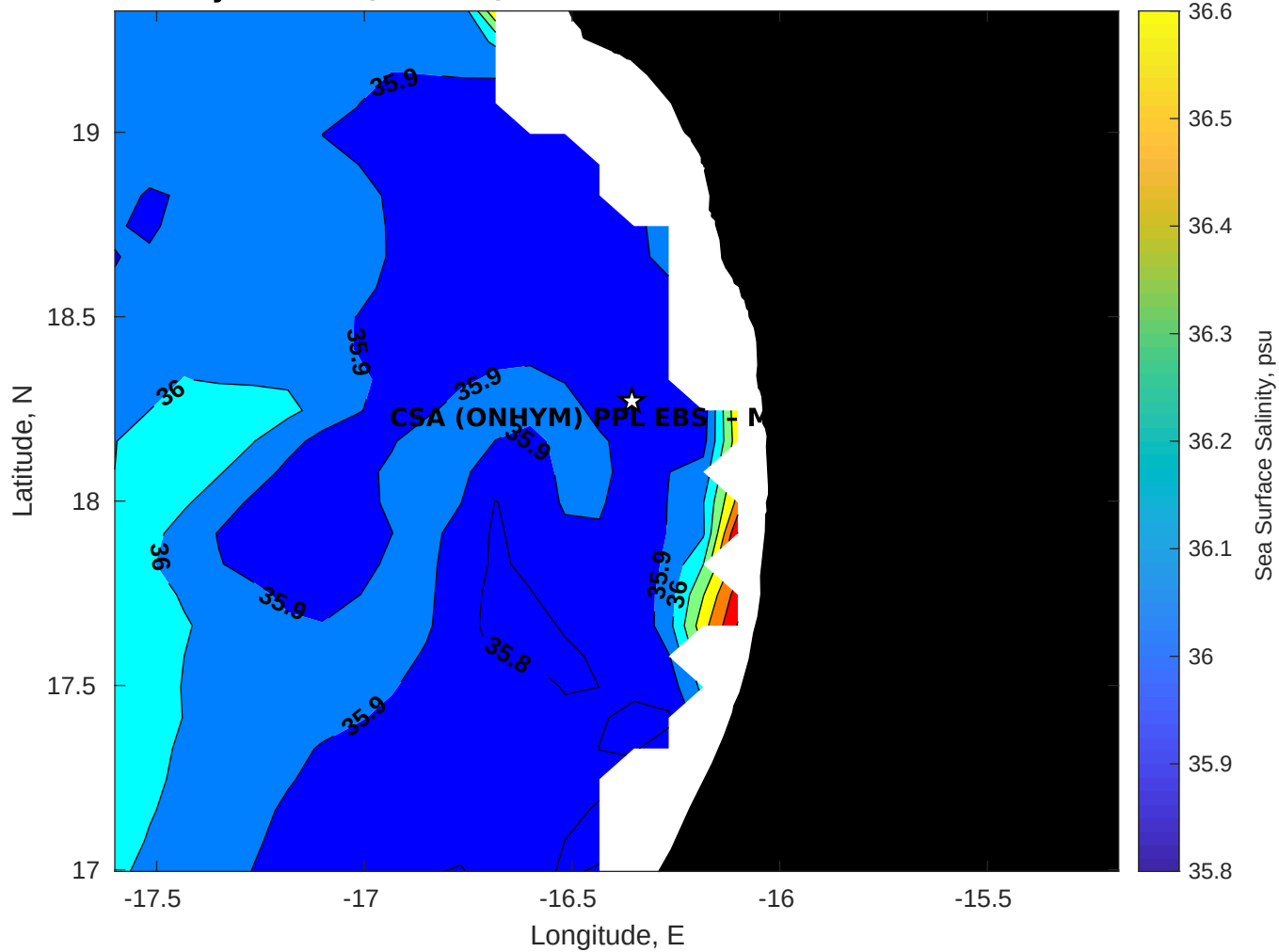
Surface Salinity for CSA (ONHYM) PPL EBS - Mauritania at 05-Feb-2026 00:00:00
