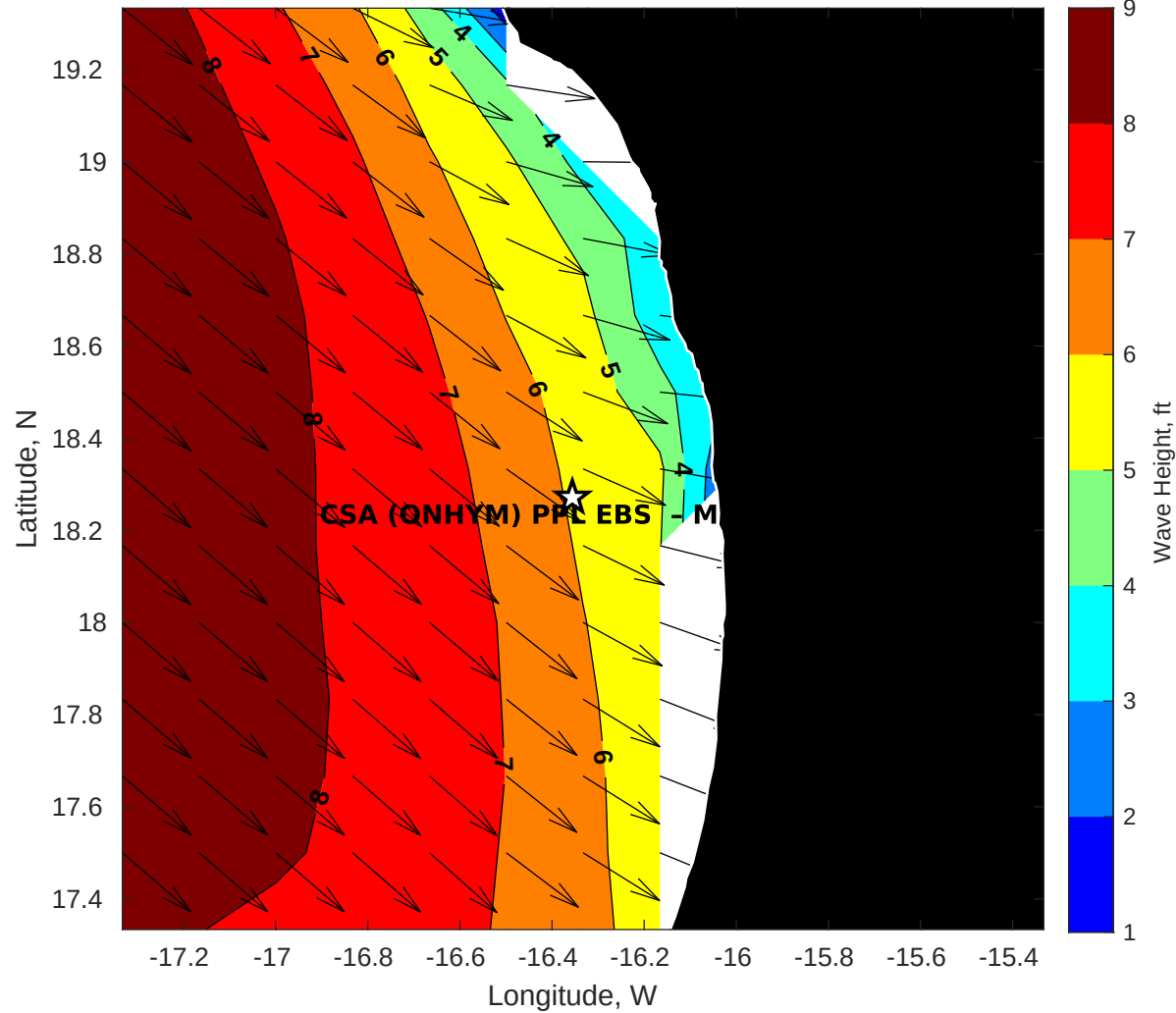
GFS Wave Height (ft) for CSA (ONHYM) PPL EBS - Mauritania at 06-Feb-2026 09:00:00
