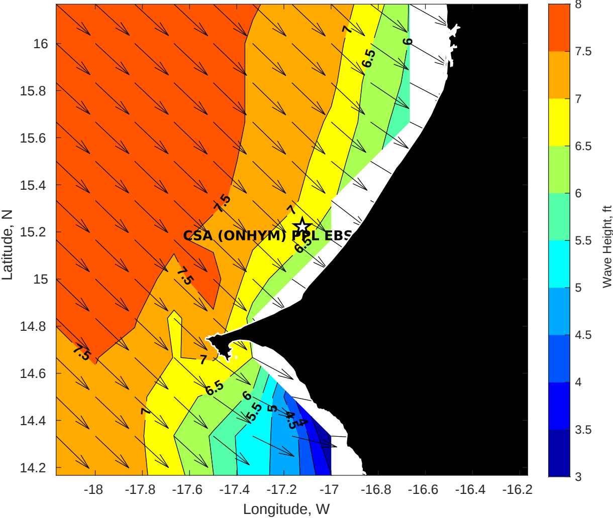
GFS Wave Height (ft) for CSA (ONHYM) PPL EBS - Senegal at 06-Feb-2026 09:00:00
